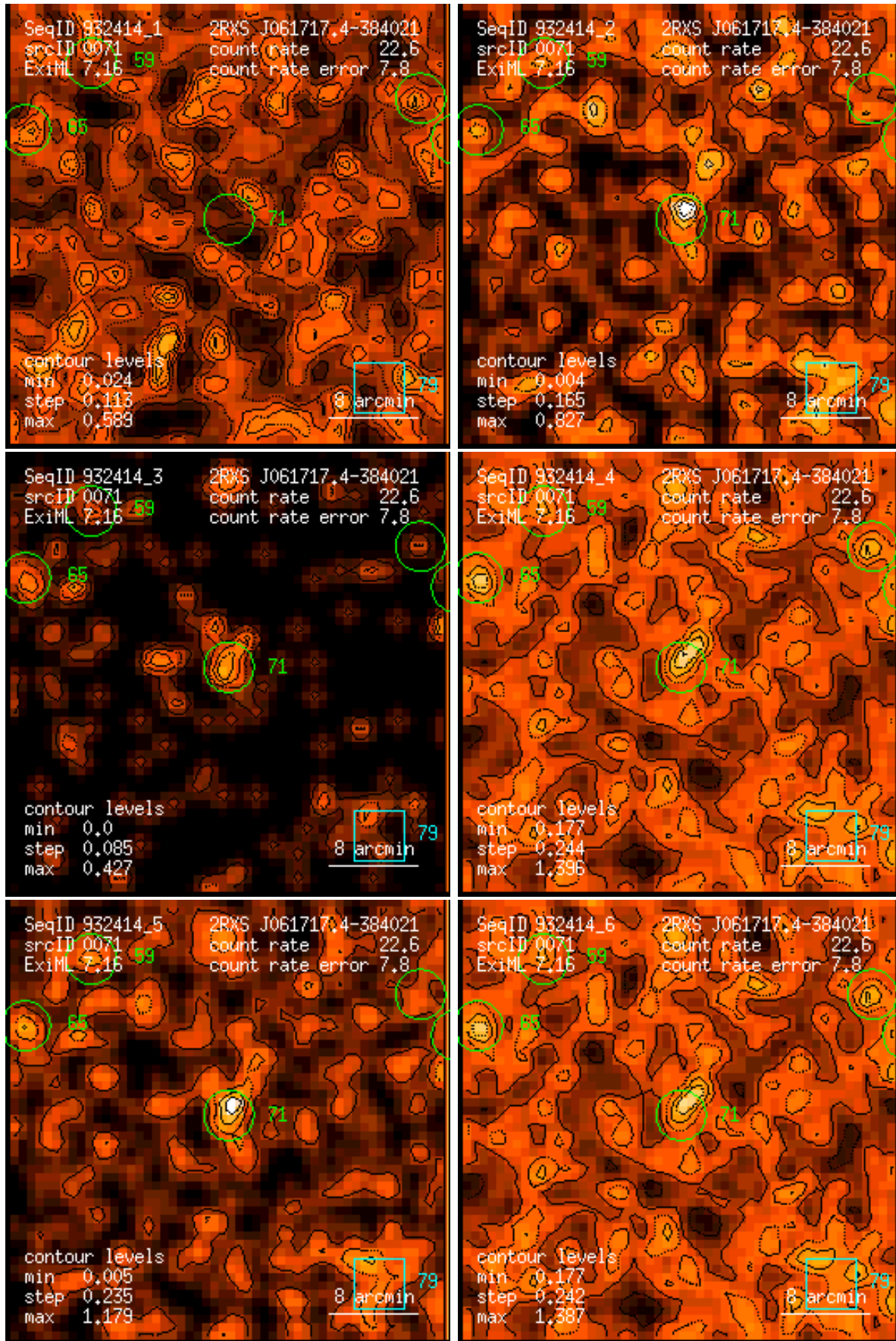
Figure 71: RASS 932414: detection 0071: band rate images, Gaussian filter: (1) PSPC channels 11 – 41, (2) 52 – 90, (3) 91 – 201, (4) 11 – 235, (5) 52 – 201, (6) 11 – 201. Broad band rates in counts/ks. Band rate contour levels in counts/ks/arcmin 2 .
