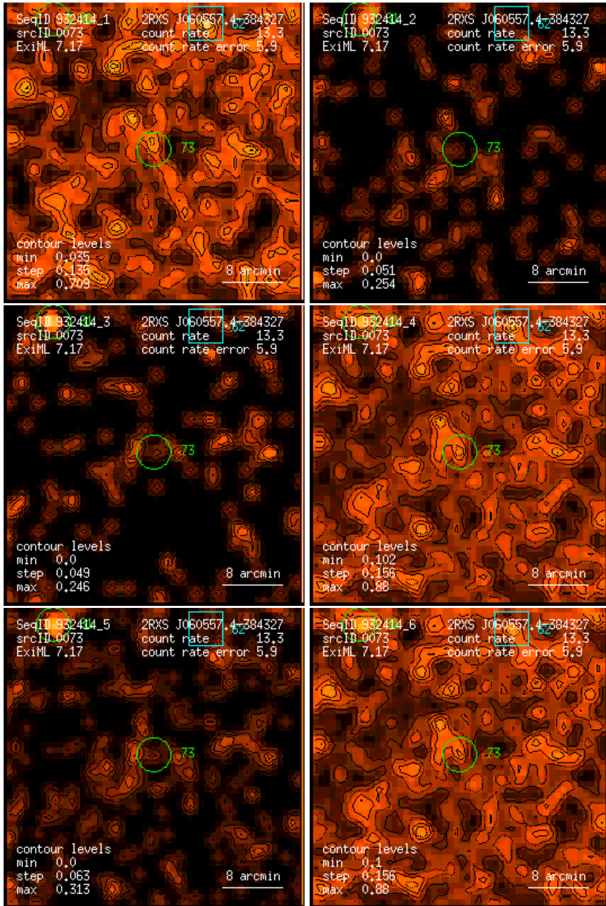
Figure 73: RASS 932414: detection 0073: band rate images, Gaussian filter: (1) PSPC channels 11 – 41, (2) 52 – 90, (3) 91 – 201, (4) 11 – 235, (5) 52 – 201, (6) 11 – 201. Broad band rates in counts/ks. Band rate contour levels in counts/ks/arcmin 2 .
