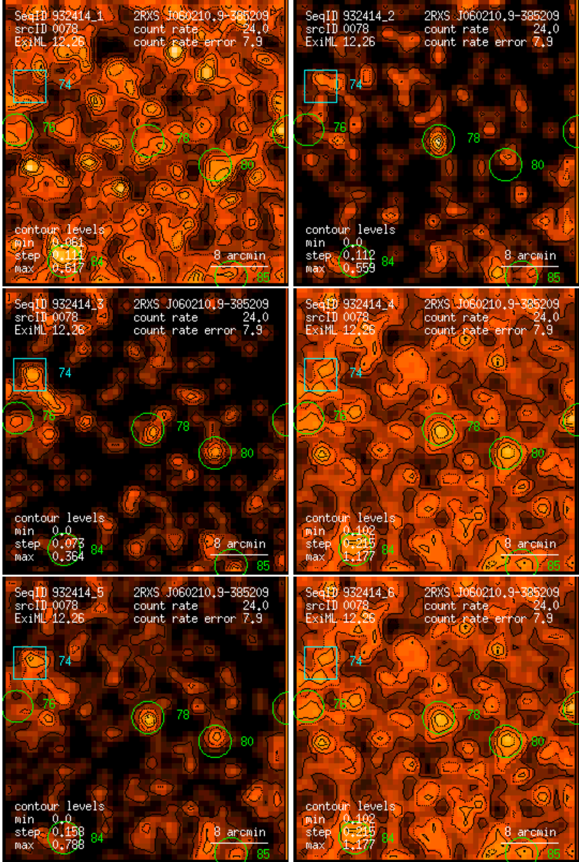
Figure 78: RASS 932414: detection 0078: band rate images, Gaussian filter: (1) PSPC channels 11 – 41, (2) 52 – 90, (3) 91 – 201, (4) 11 – 235, (5) 52 – 201, (6) 11 – 201. Broad band rates in counts/ks. Band rate contour levels in counts/ks/arcmin 2 .
