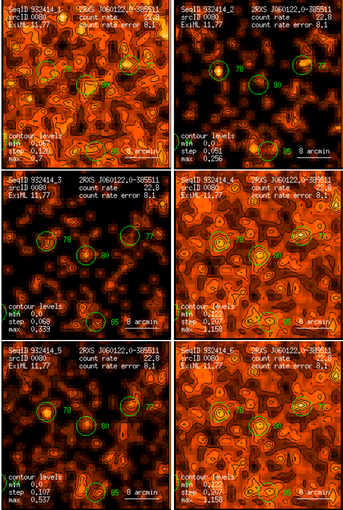
Figure 80: RASS 932414: detection 0080: band rate images, Gaussian filter: (1) PSPC channels 11 – 41, (2) 52 – 90, (3) 91 – 201, (4) 11 – 235, (5) 52 – 201, (6) 11 – 201. Broad band rates in counts/ks. Band rate contour levels in counts/ks/arcmin 2 .
