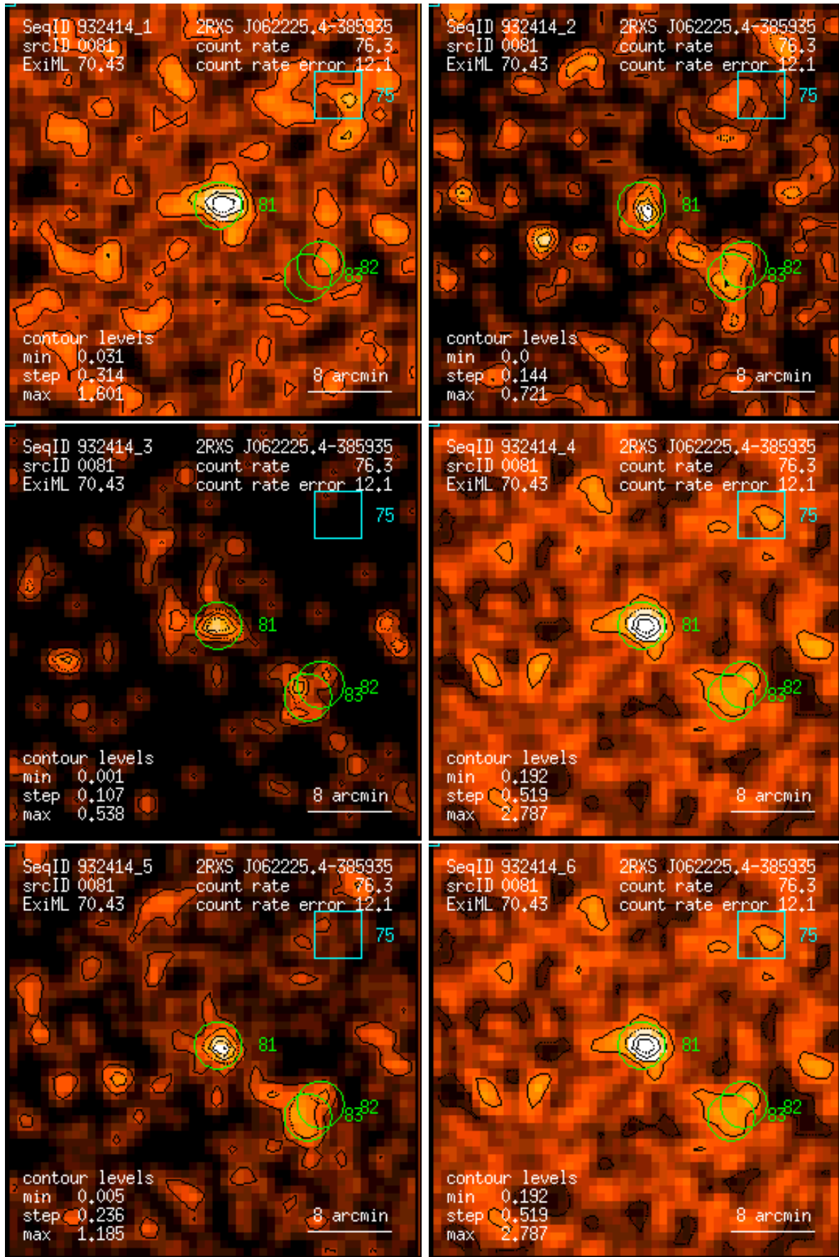
Figure 81: RASS 932414: detection 0081: band rate images, Gaussian filter: (1) PSPC channels 11 – 41, (2) 52 – 90, (3) 91 – 201, (4) 11 – 235, (5) 52 – 201, (6) 11 – 201. Broad band rates in counts/ks. Band rate contour levels in counts/ks/arcmin 2 .
