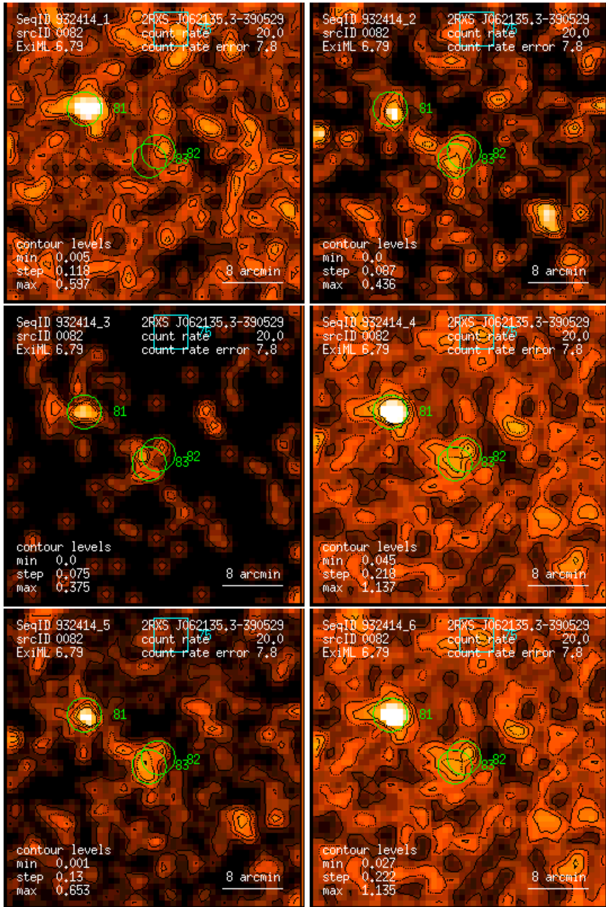
Figure 82: RASS 932414: detection 0082: band rate images, Gaussian filter: (1) PSPC channels 11 – 41, (2) 52 – 90, (3) 91 – 201, (4) 11 – 235, (5) 52 – 201, (6) 11 – 201. Broad band rates in counts/ks. Band rate contour levels in counts/ks/arcmin 2 .
