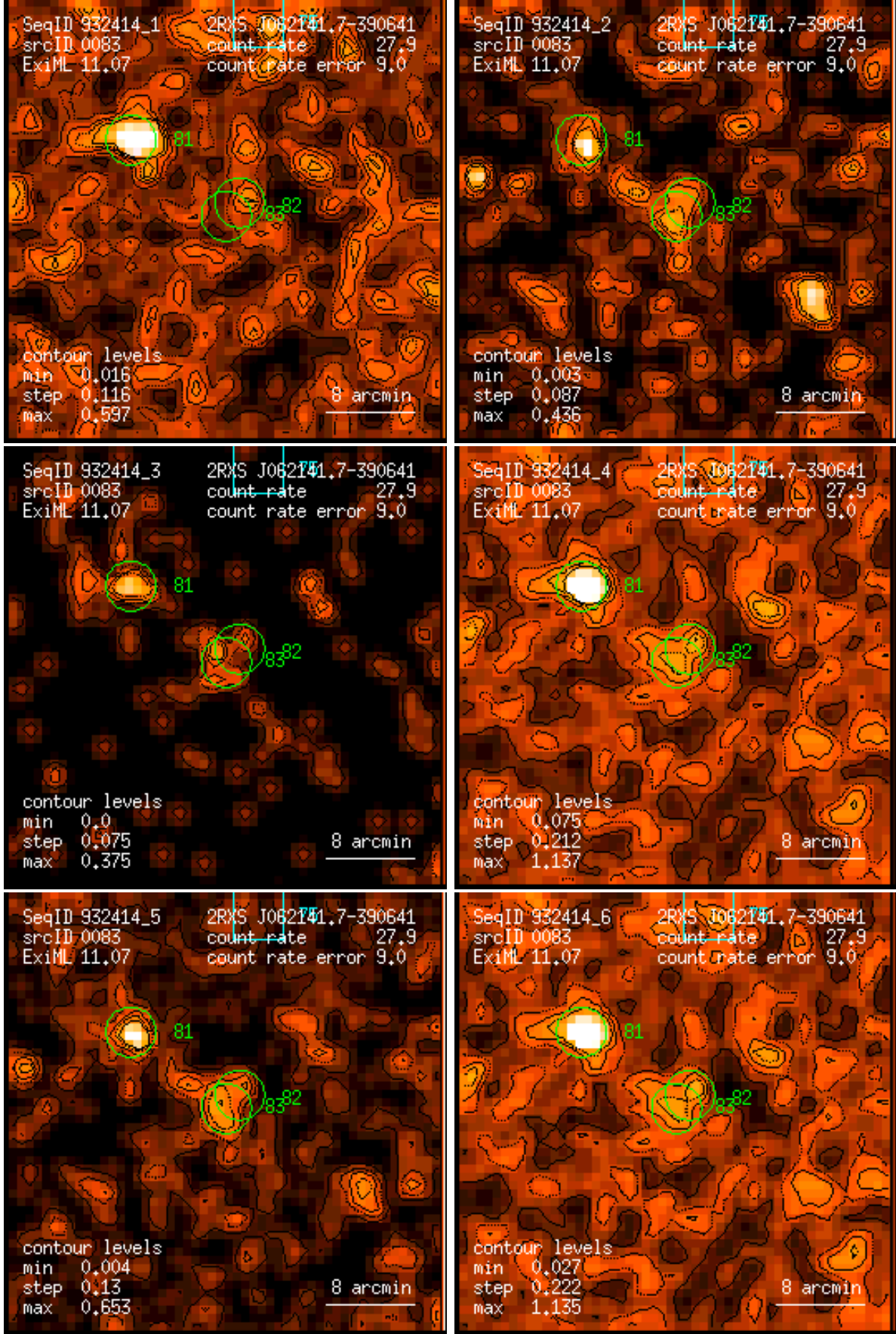
Figure 83: RASS 932414: detection 0083: band rate images, Gaussian filter: (1) PSPC channels 11 – 41, (2) 52 – 90, (3) 91 – 201, (4) 11 – 235, (5) 52 – 201, (6) 11 – 201. Broad band rates in counts/ks. Band rate contour levels in counts/ks/arcmin 2 .
