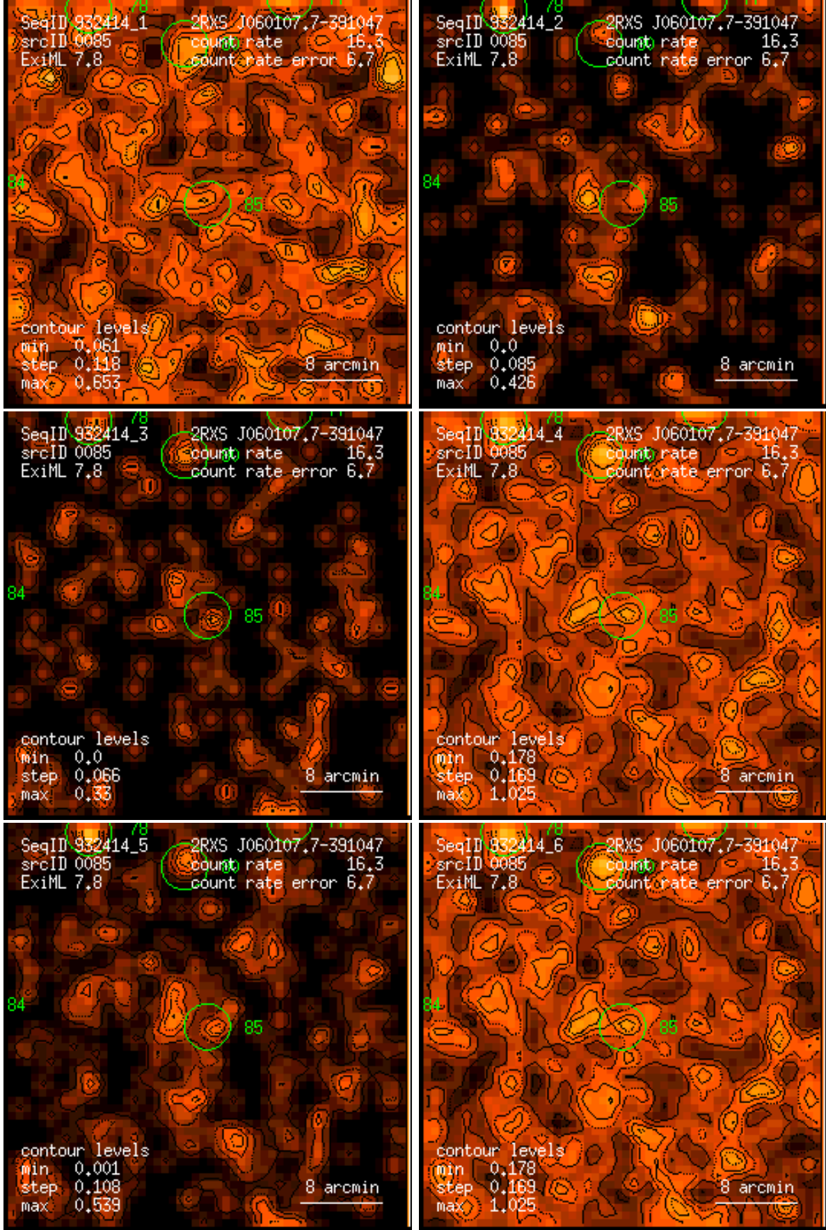
Figure 85: RASS 932414: detection 0085: band rate images, Gaussian filter: (1) PSPC channels 11 – 41, (2) 52 – 90, (3) 91 – 201, (4) 11 – 235, (5) 52 – 201, (6) 11 – 201. Broad band rates in counts/ks. Band rate contour levels in counts/ks/arcmin 2 .
