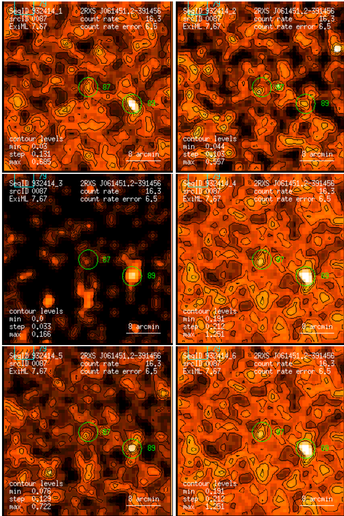
Figure 87: RASS 932414: detection 0087: band rate images, Gaussian filter: (1) PSPC channels 11 – 41, (2) 52 – 90, (3) 91 – 201, (4) 11 – 235, (5) 52 – 201, (6) 11 – 201. Broad band rates in counts/ks. Band rate contour levels in counts/ks/arcmin 2 .
