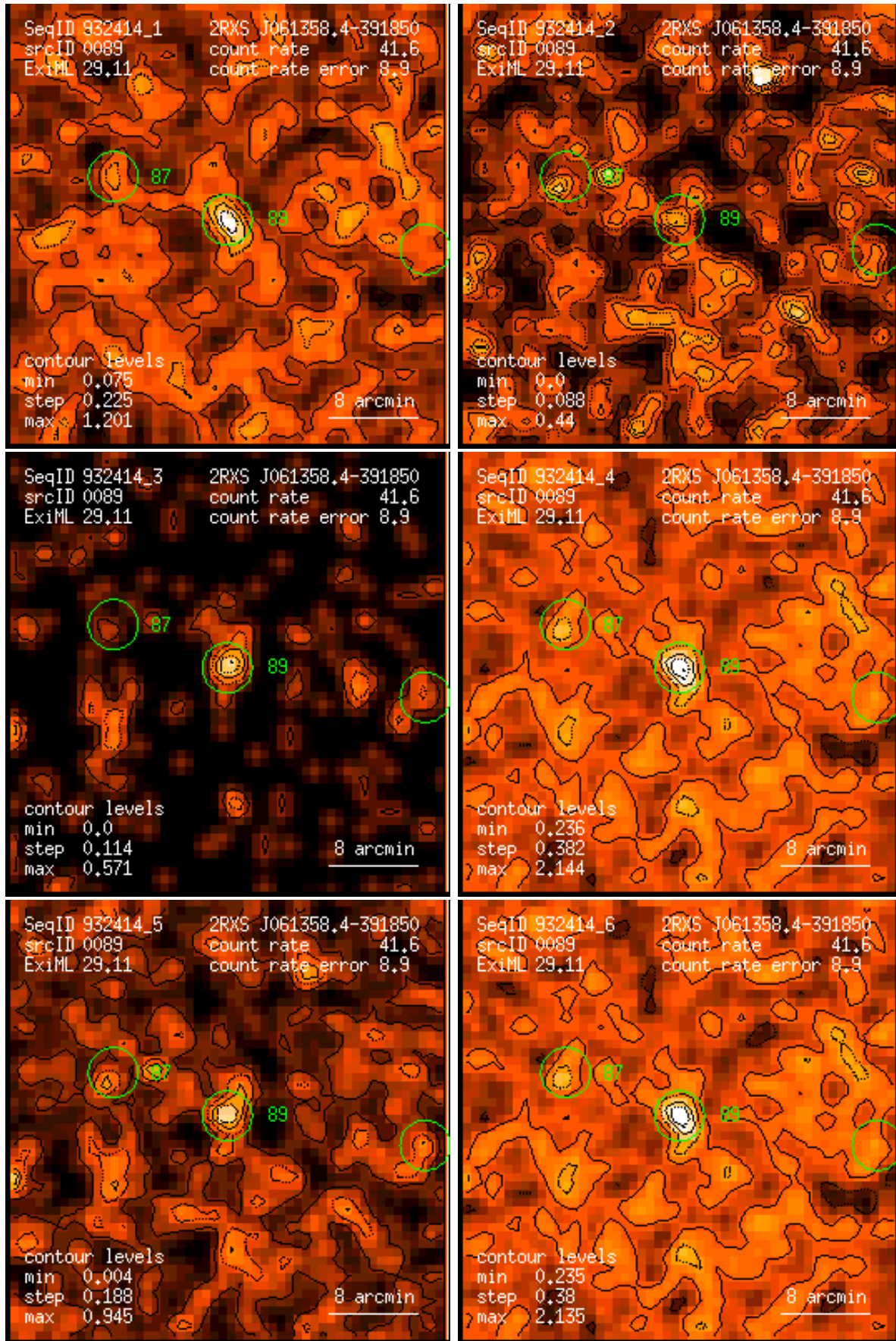
Figure 89: RASS 932414: detection 0089: band rate images, Gaussian filter: (1) PSPC channels 11 – 41, (2) 52 – 90, (3) 91 – 201, (4) 11 – 235, (5) 52 – 201, (6) 11 – 201. Broad band rates in counts/ks. Band rate contour levels in counts/ks/arcmin 2 .
