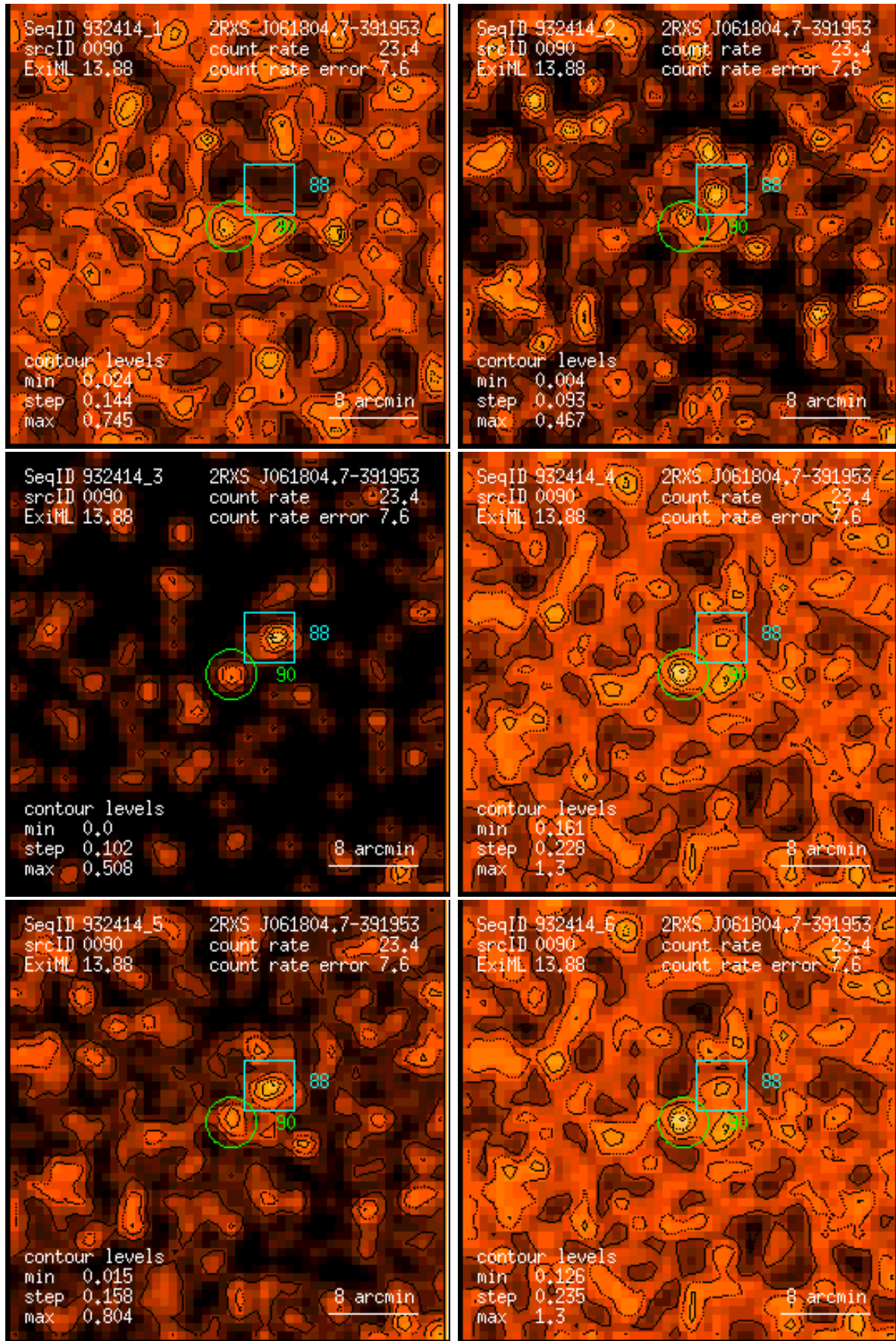
Figure 90: RASS 932414: detection 0090: band rate images, Gaussian filter: (1) PSPC channels 11 – 41, (2) 52 – 90, (3) 91 – 201, (4) 11 – 235, (5) 52 – 201, (6) 11 – 201. Broad band rates in counts/ks. Band rate contour levels in counts/ks/arcmin 2 .
