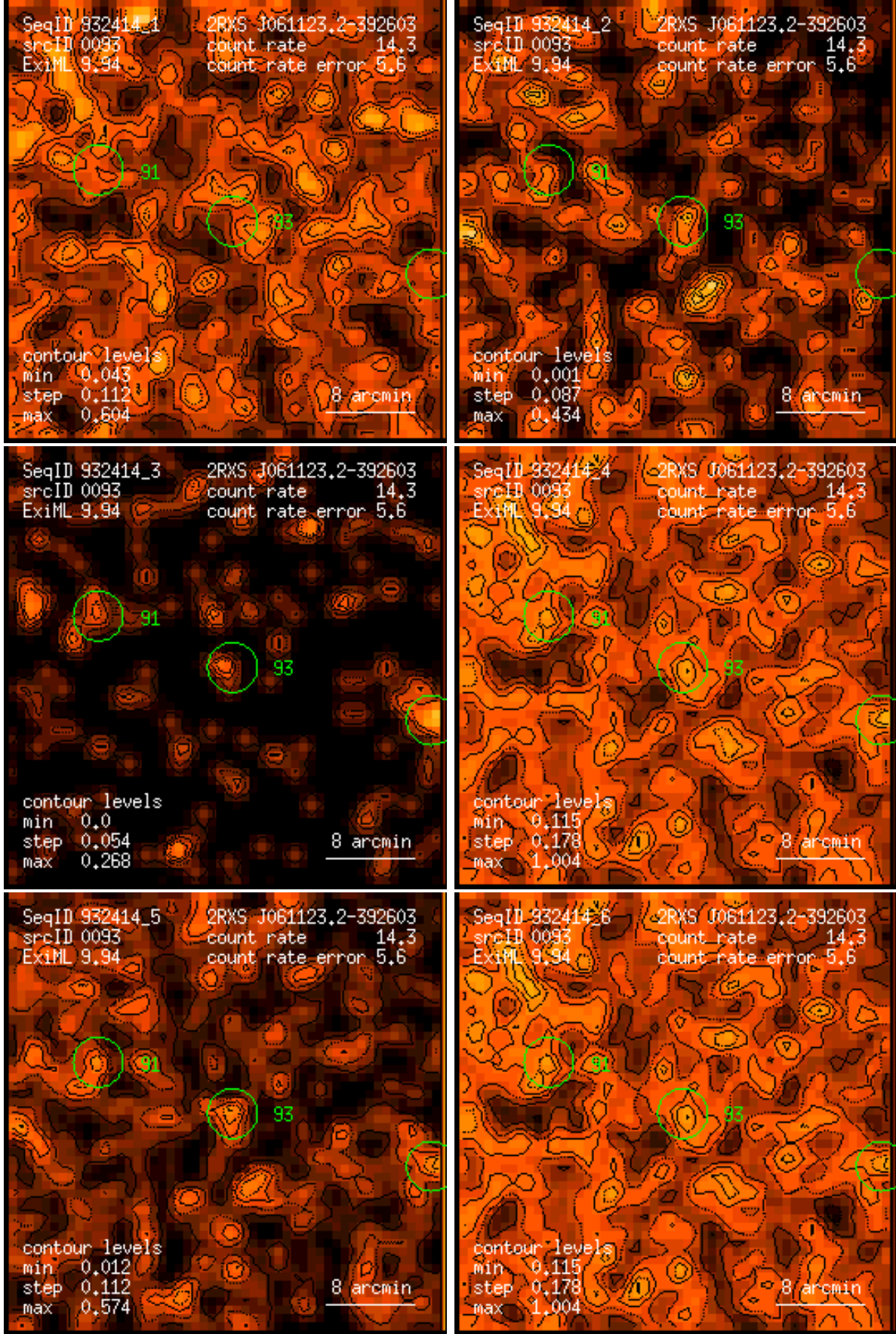
Figure 93: RASS 932414: detection 0093: band rate images, Gaussian filter: (1) PSPC channels 11 – 41, (2) 52 – 90, (3) 91 – 201, (4) 11 – 235, (5) 52 – 201, (6) 11 – 201. Broad band rates in counts/ks. Band rate contour levels in counts/ks/arcmin 2 .
