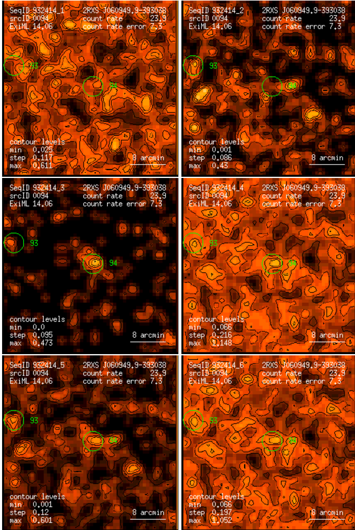
Figure 94: RASS 932414: detection 0094: band rate images, Gaussian filter: (1) PSPC channels 11 – 41, (2) 52 – 90, (3) 91 – 201, (4) 11 – 235, (5) 52 – 201, (6) 11 – 201. Broad band rates in counts/ks. Band rate contour levels in counts/ks/arcmin 2 .
