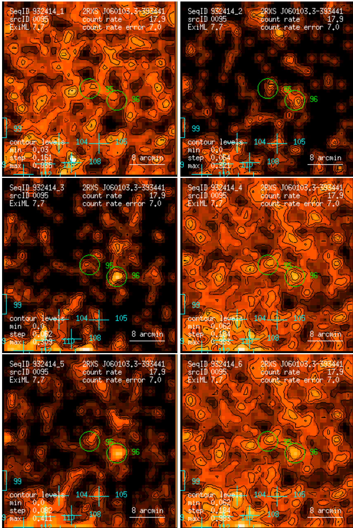
Figure 95: RASS 932414: detection 0095: band rate images, Gaussian filter: (1) PSPC channels 11 – 41, (2) 52 – 90, (3) 91 – 201, (4) 11 – 235, (5) 52 – 201, (6) 11 – 201. Broad band rates in counts/ks. Band rate contour levels in counts/ks/arcmin 2 .
