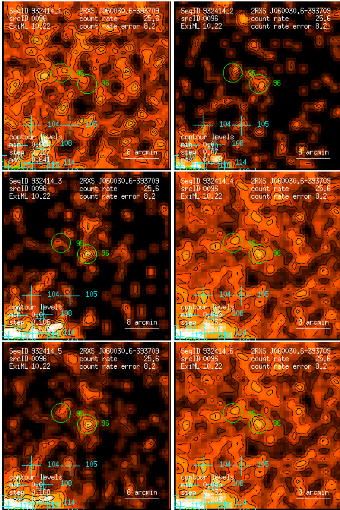
Figure 96: RASS 932414: detection 0096: band rate images, Gaussian filter: (1) PSPC channels 11 – 41, (2) 52 – 90, (3) 91 – 201, (4) 11 – 235, (5) 52 – 201, (6) 11 – 201. Broad band rates in counts/ks. Band rate contour levels in counts/ks/arcmin 2 .
