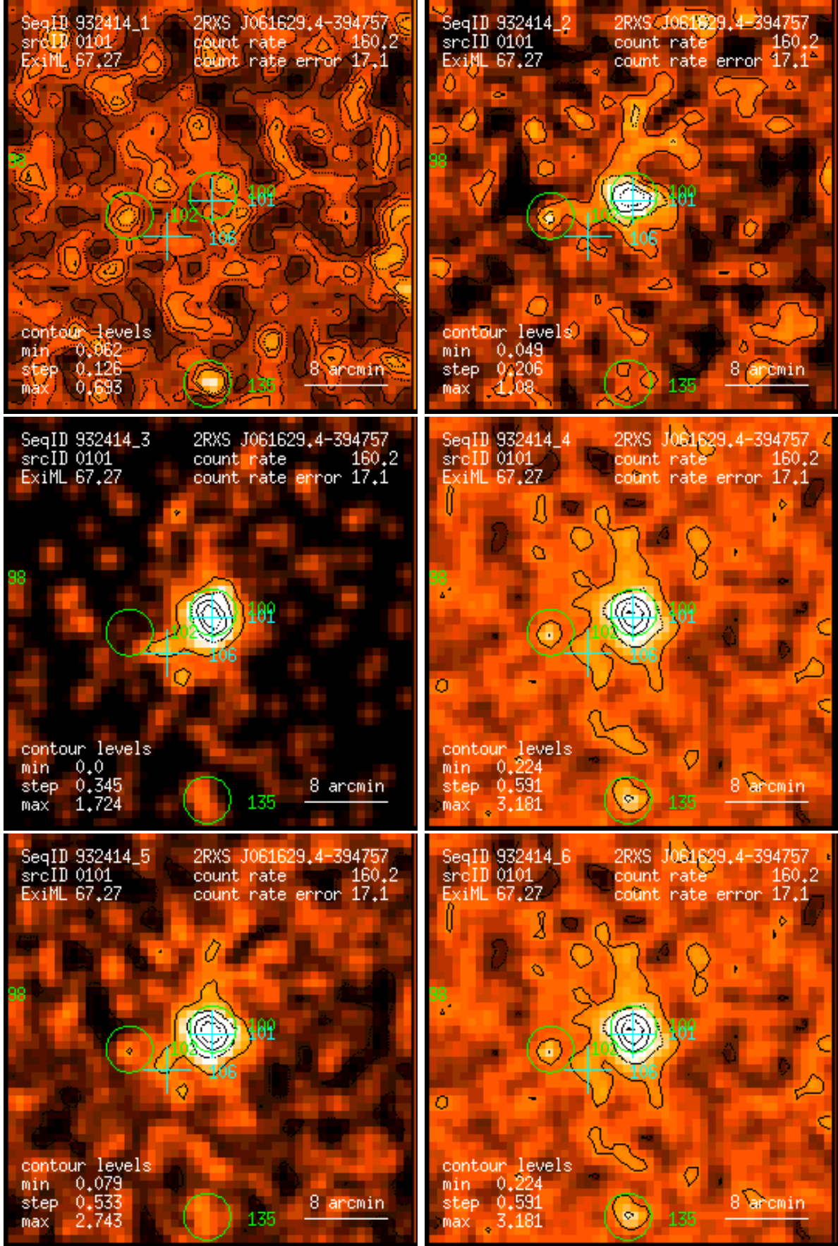
Figure 101: RASS 932414: detection 0101: band rate images, Gaussian filter: (1) PSPC channels 11 – 41, (2) 52 – 90, (3) 91 – 201, (4) 11 – 235, (5) 52 – 201, (6) 11 – 201. Broad band rates in counts/ks. Band rate contour levels in counts/ks/arcmin 2 .
