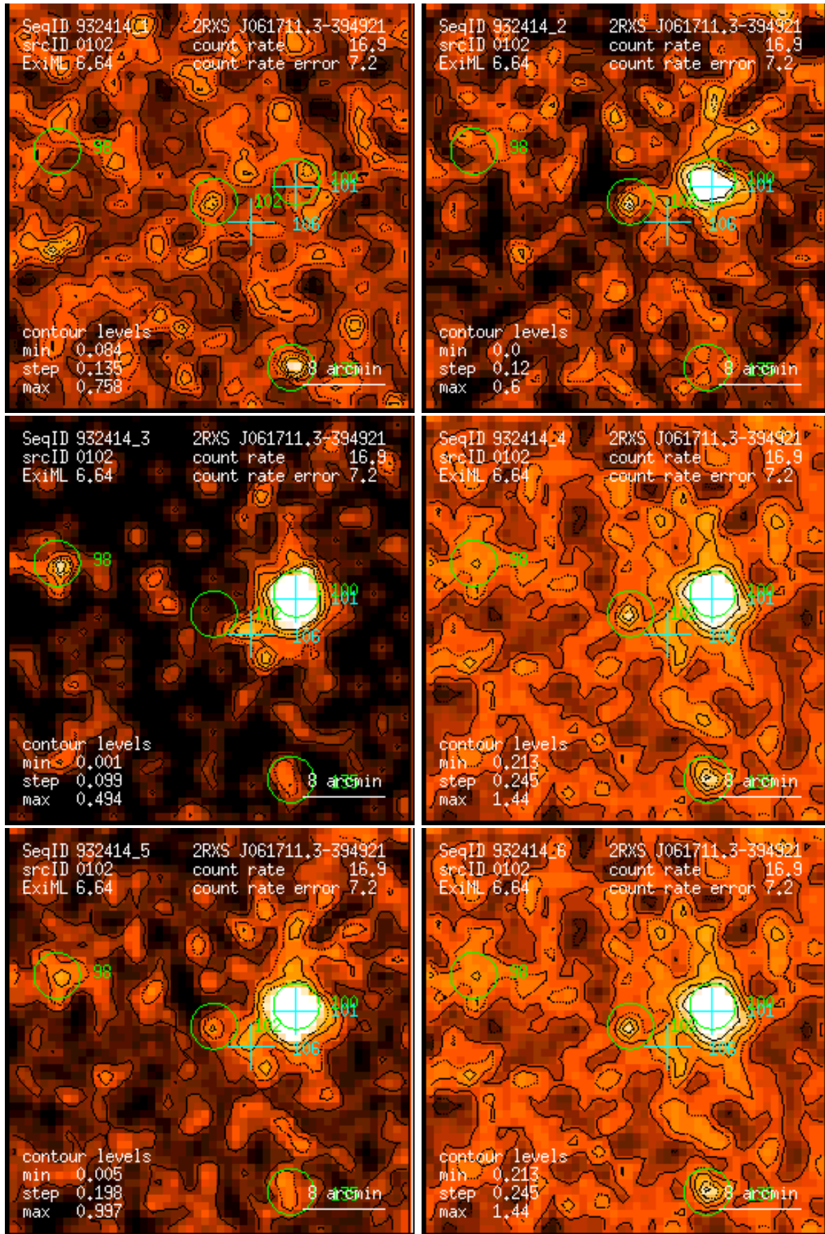
Figure 102: RASS 932414: detection 0102: band rate images, Gaussian filter: (1) PSPC channels 11 – 41, (2) 52 – 90, (3) 91 – 201, (4) 11 – 235, (5) 52 – 201, (6) 11 – 201. Broad band rates in counts/ks. Band rate contour levels in counts/ks/arcmin 2 .
