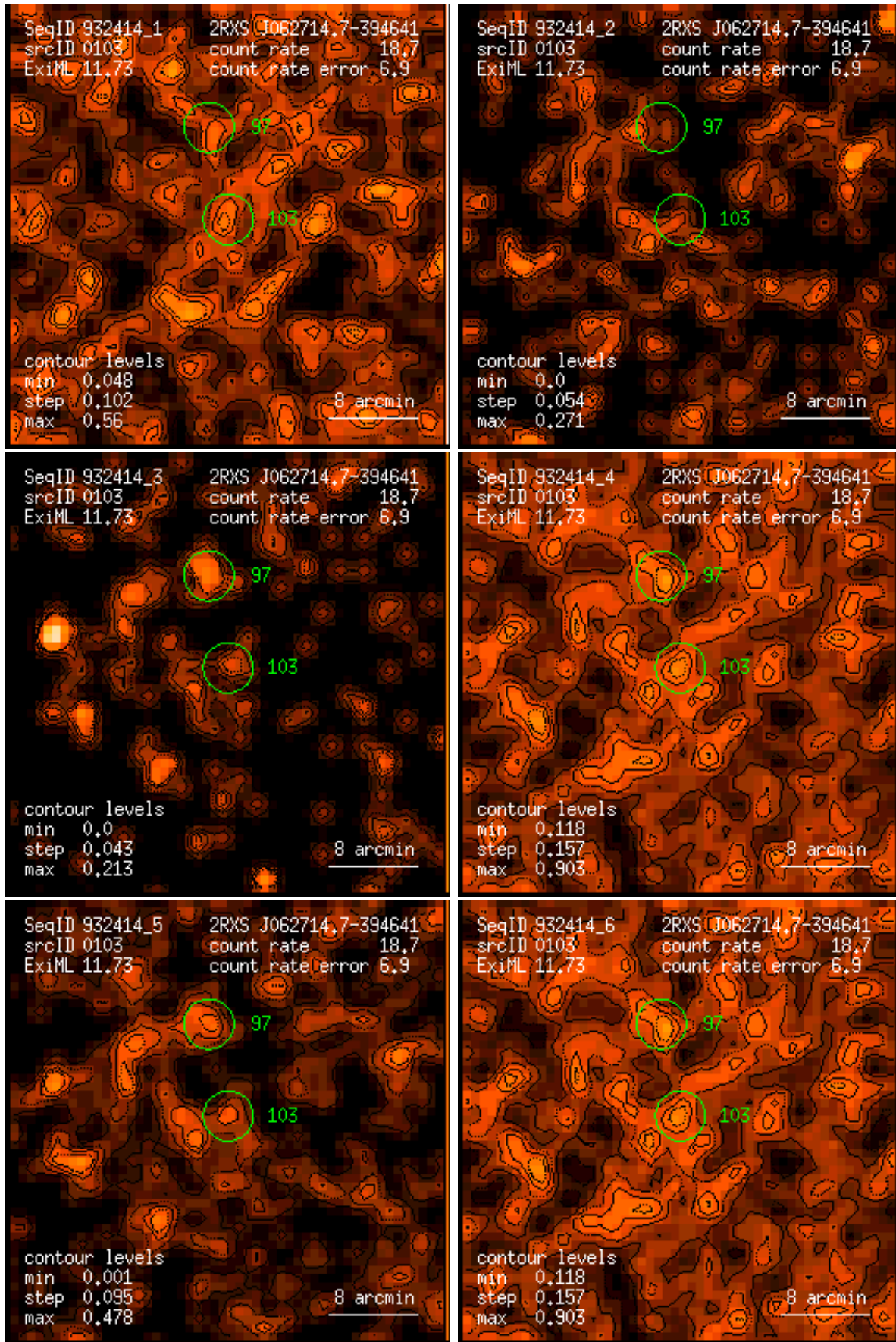
Figure 103: RASS 932414: detection 0103: band rate images, Gaussian filter: (1) PSPC channels 11 – 41, (2) 52 – 90, (3) 91 – 201, (4) 11 – 235, (5) 52 – 201, (6) 11 – 201. Broad band rates in counts/ks. Band rate contour levels in counts/ks/arcmin 2 .
