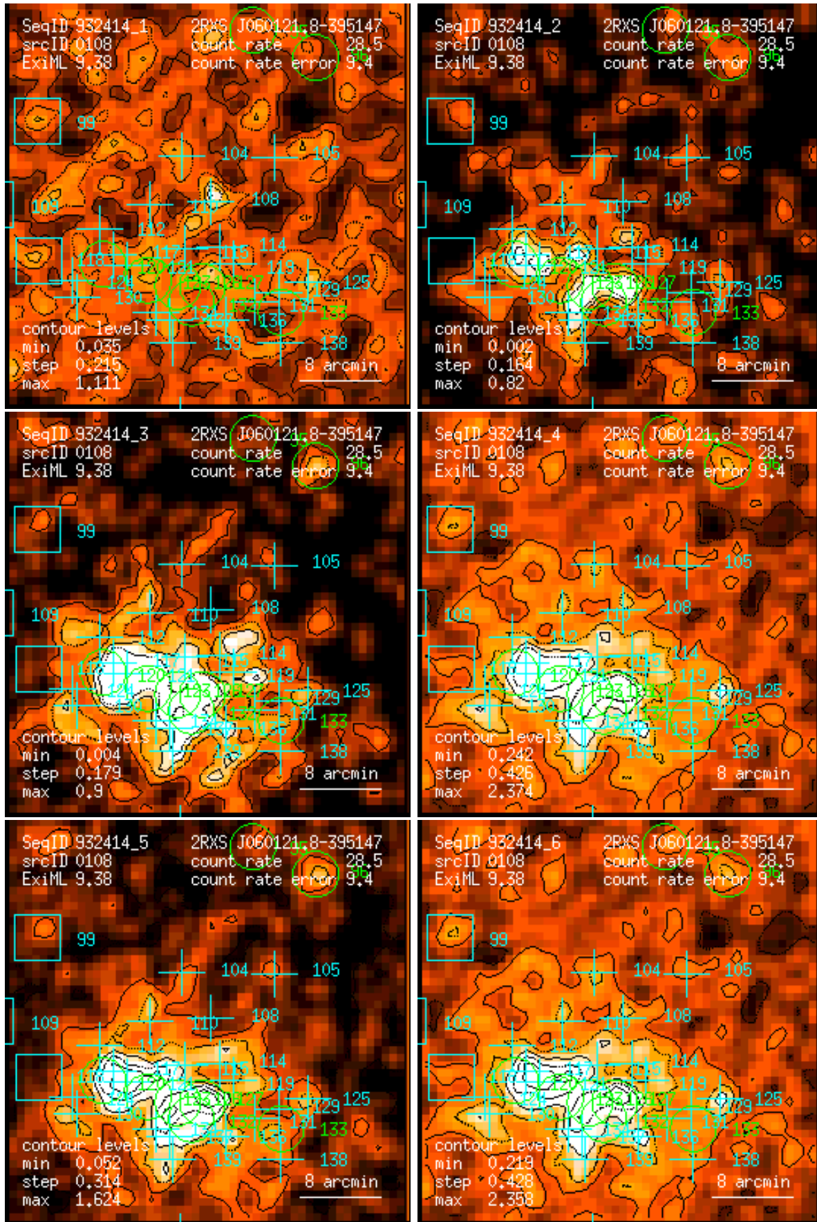
Figure 108: RASS 932414: detection 0108: band rate images, Gaussian filter: (1) PSPC channels 11 – 41, (2) 52 – 90, (3) 91 – 201, (4) 11 – 235, (5) 52 – 201, (6) 11 – 201. Broad band rates in counts/ks. Band rate contour levels in counts/ks/arcmin 2 .
