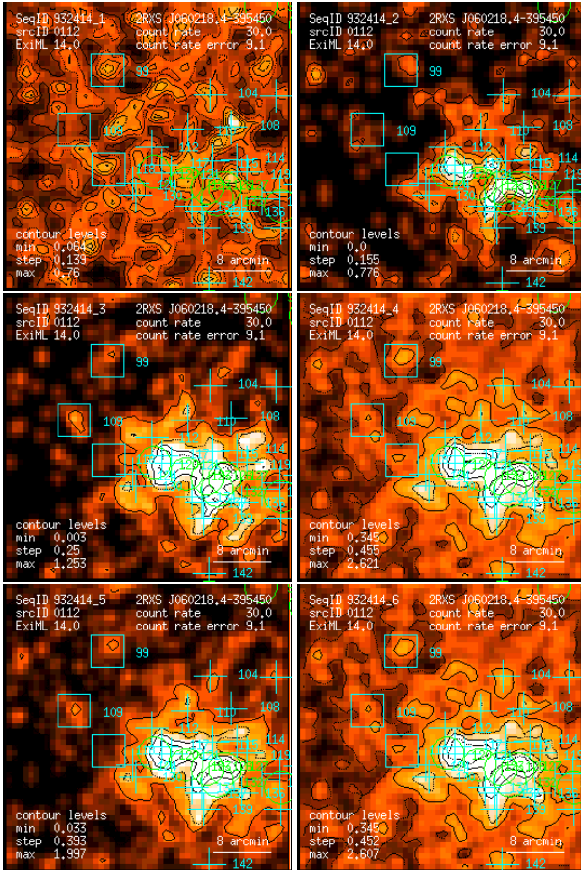
Figure 112: RASS 932414: detection 0112: band rate images, Gaussian filter: (1) PSPC channels 11 – 41, (2) 52 – 90, (3) 91 – 201, (4) 11 – 235, (5) 52 – 201, (6) 11 – 201. Broad band rates in counts/ks. Band rate contour levels in counts/ks/arcmin 2 .
