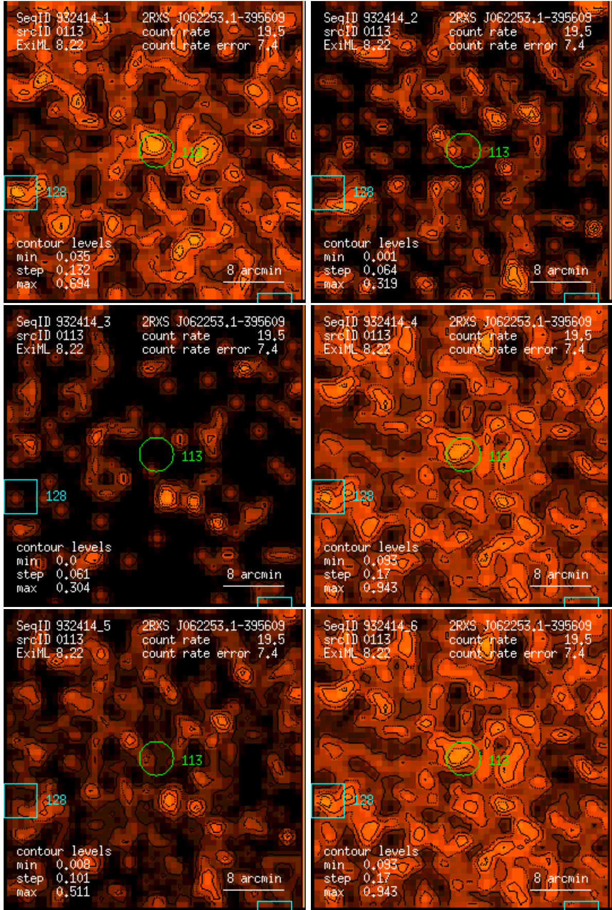
Figure 113: RASS 932414: detection 0113: band rate images, Gaussian filter: (1) PSPC channels 11 – 41, (2) 52 – 90, (3) 91 – 201, (4) 11 – 235, (5) 52 – 201, (6) 11 – 201. Broad band rates in counts/ks. Band rate contour levels in counts/ks/arcmin 2 .
