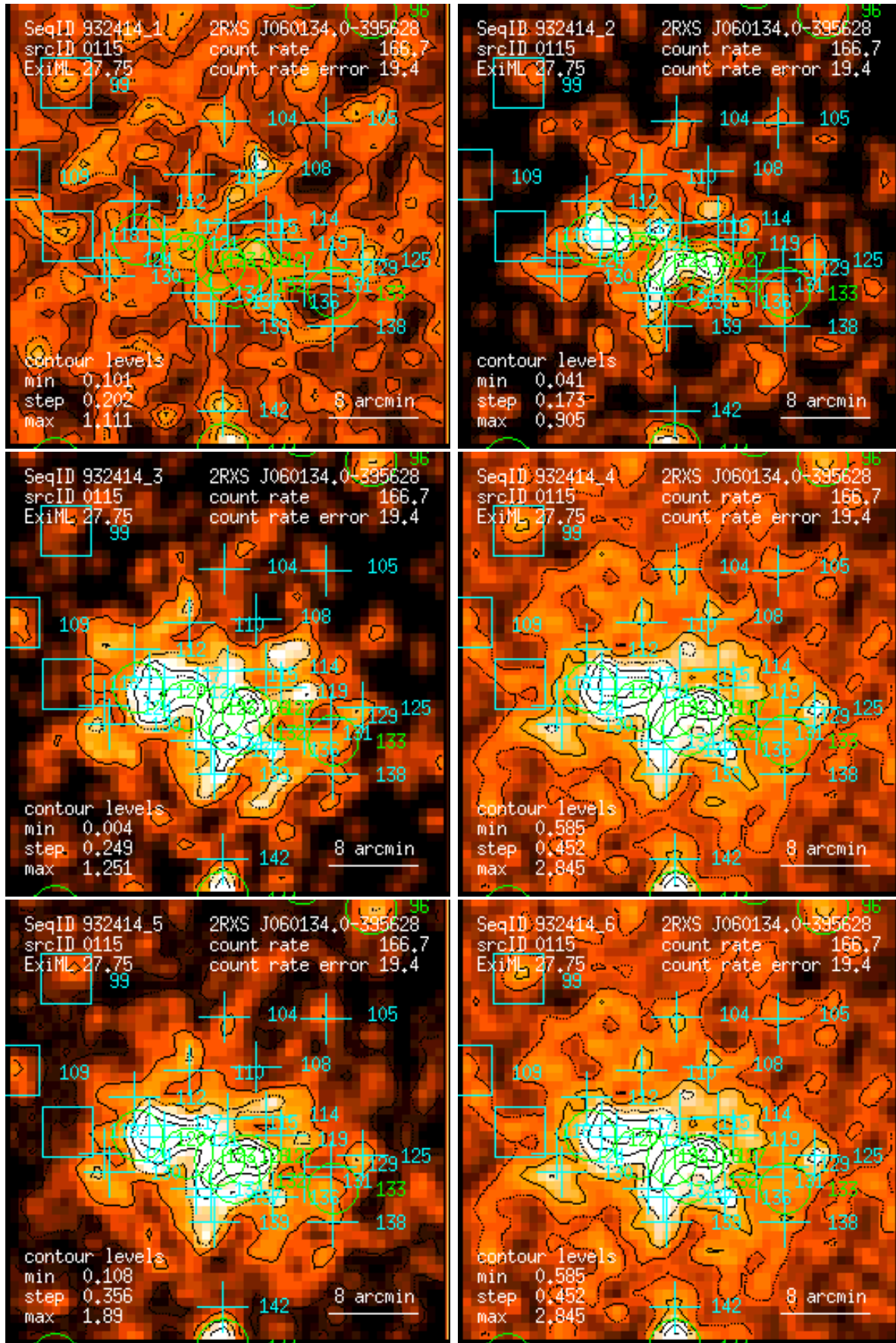
Figure 115: RASS 932414: detection 0115: band rate images, Gaussian filter: (1) PSPC channels 11 – 41, (2) 52 – 90, (3) 91 – 201, (4) 11 – 235, (5) 52 – 201, (6) 11 – 201. Broad band rates in counts/ks. Band rate contour levels in counts/ks/arcmin 2 .
