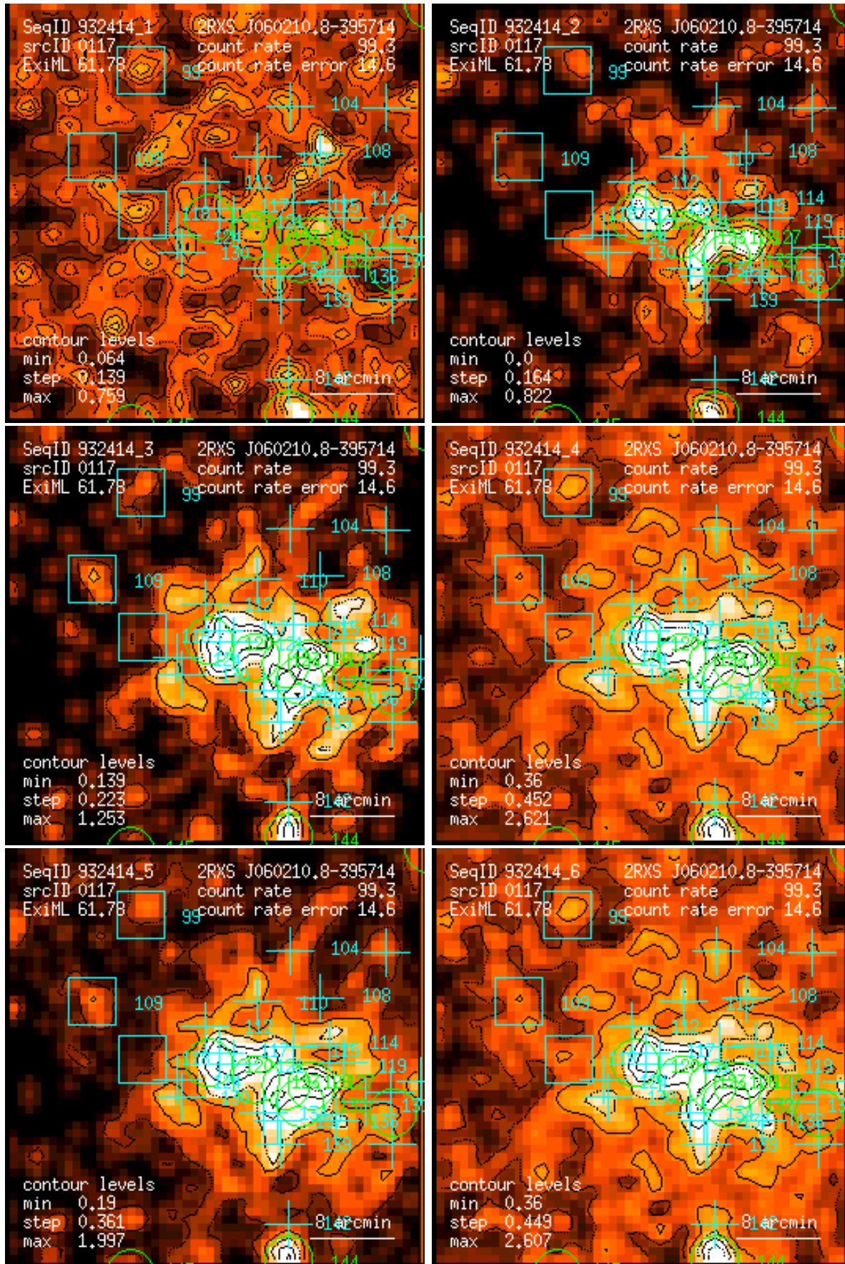
Figure 117: RASS 932414: detection 0117: band rate images, Gaussian filter: (1) PSPC channels 11 – 41, (2) 52 – 90, (3) 91 – 201, (4) 11 – 235, (5) 52 – 201, (6) 11 – 201. Broad band rates in counts/ks. Band rate contour levels in counts/ks/arcmin 2 .
