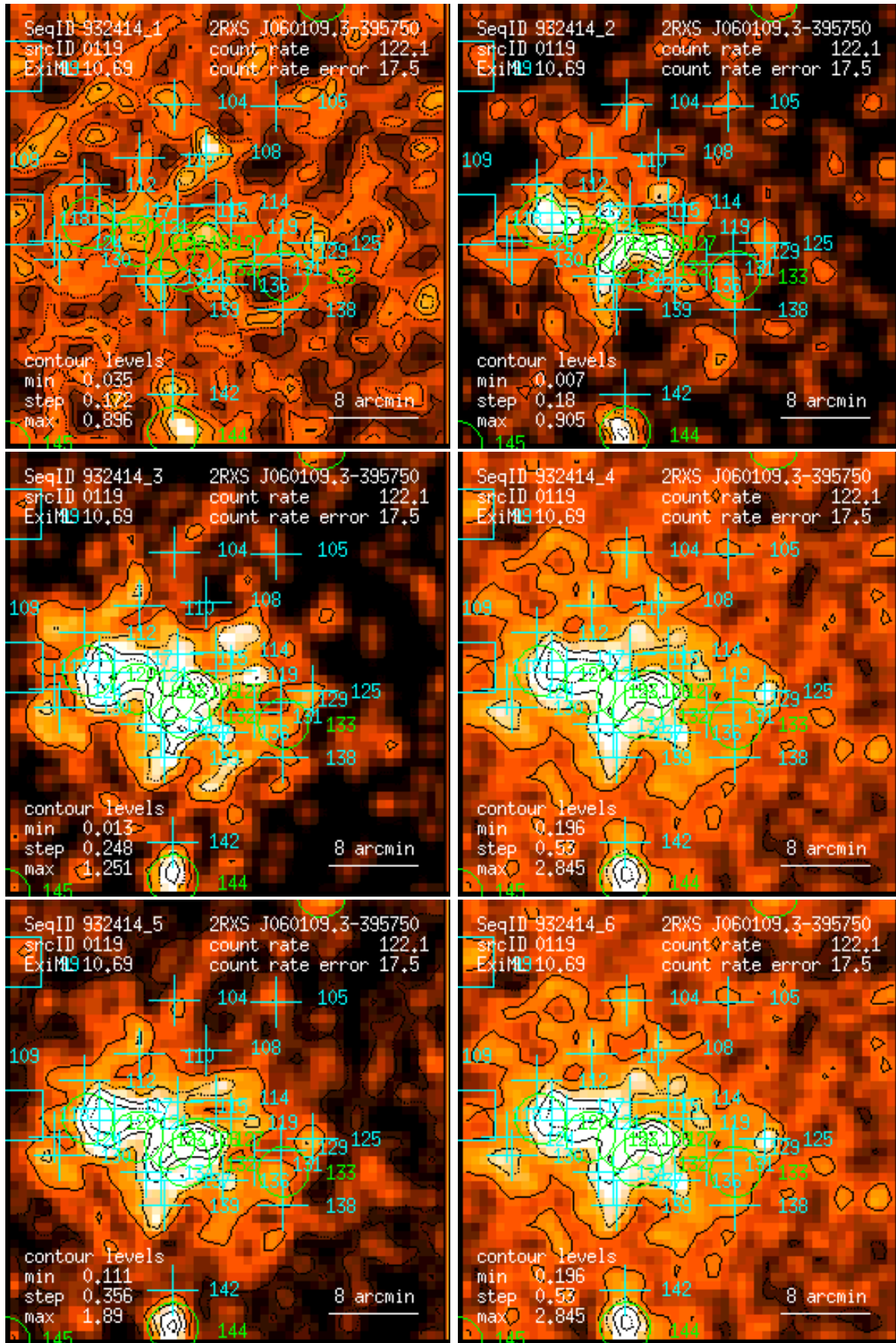
Figure 119: RASS 932414: detection 0119: band rate images, Gaussian filter: (1) PSPC channels 11 – 41, (2) 52 – 90, (3) 91 – 201, (4) 11 – 235, (5) 52 – 201, (6) 11 – 201. Broad band rates in counts/ks. Band rate contour levels in counts/ks/arcmin 2 .
