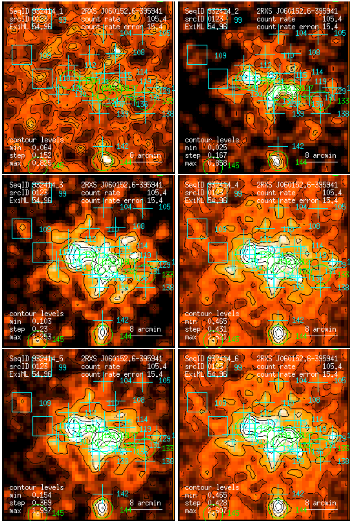
Figure 123: RASS 932414: detection 0123: band rate images, Gaussian filter: (1) PSPC channels 11 – 41, (2) 52 – 90, (3) 91 – 201, (4) 11 – 235, (5) 52 – 201, (6) 11 – 201. Broad band rates in counts/ks. Band rate contour levels in counts/ks/arcmin 2 .
