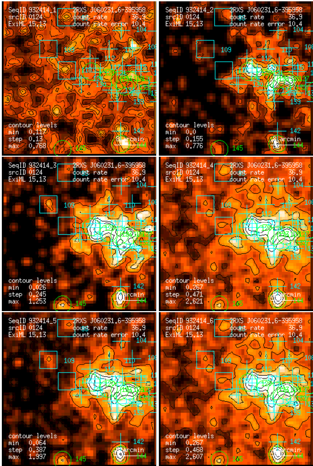
Figure 124: RASS 932414: detection 0124: band rate images, Gaussian filter: (1) PSPC channels 11 – 41, (2) 52 – 90, (3) 91 – 201, (4) 11 – 235, (5) 52 – 201, (6) 11 – 201. Broad band rates in counts/ks. Band rate contour levels in counts/ks/arcmin 2 .
