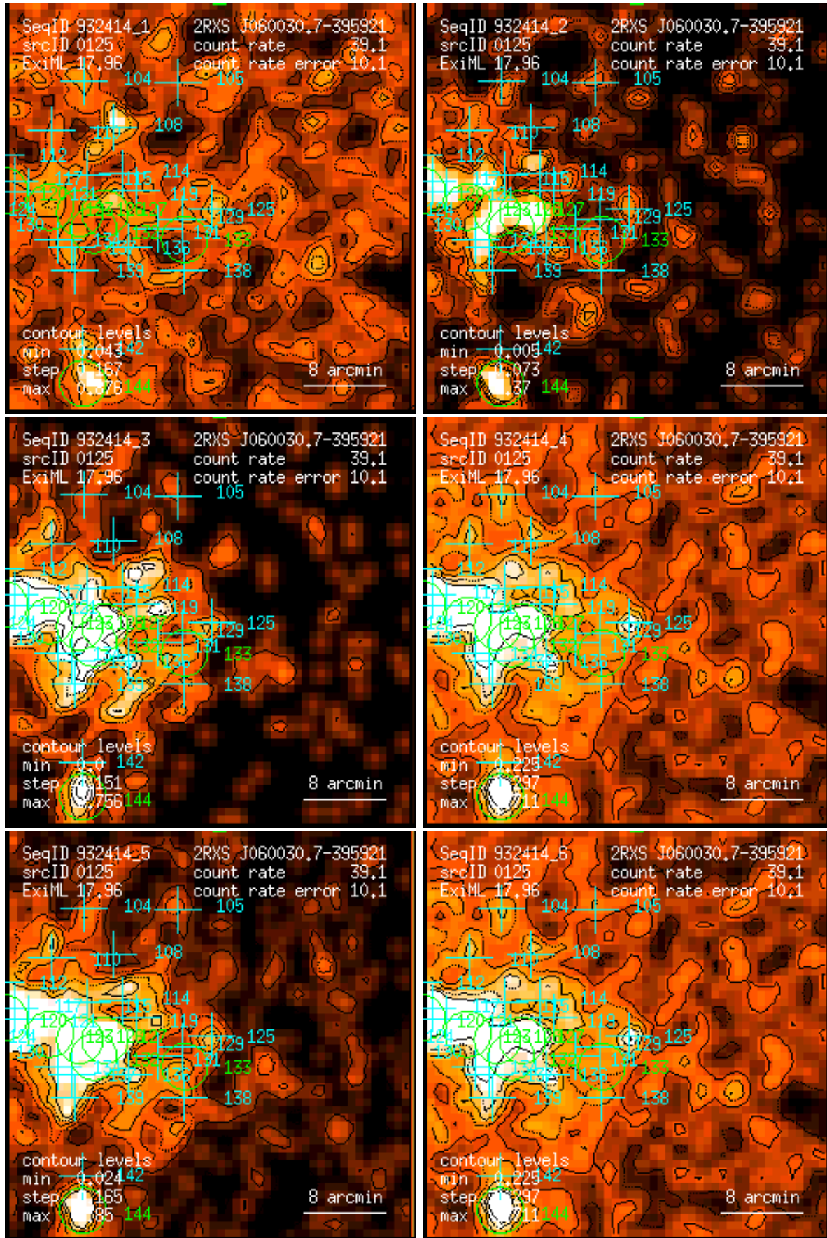
Figure 125: RASS 932414: detection 0125: band rate images, Gaussian filter: (1) PSPC channels 11 – 41, (2) 52 – 90, (3) 91 – 201, (4) 11 – 235, (5) 52 – 201, (6) 11 – 201. Broad band rates in counts/ks. Band rate contour levels in counts/ks/arcmin 2 .
