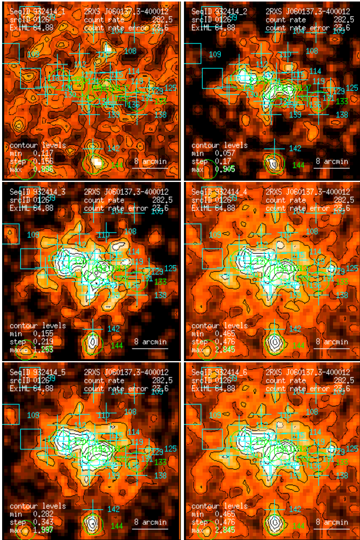
Figure 126: RASS 932414: detection 0126: band rate images, Gaussian filter: (1) PSPC channels 11 – 41, (2) 52 – 90, (3) 91 – 201, (4) 11 – 235, (5) 52 – 201, (6) 11 – 201. Broad band rates in counts/ks. Band rate contour levels in counts/ks/arcmin 2 .
