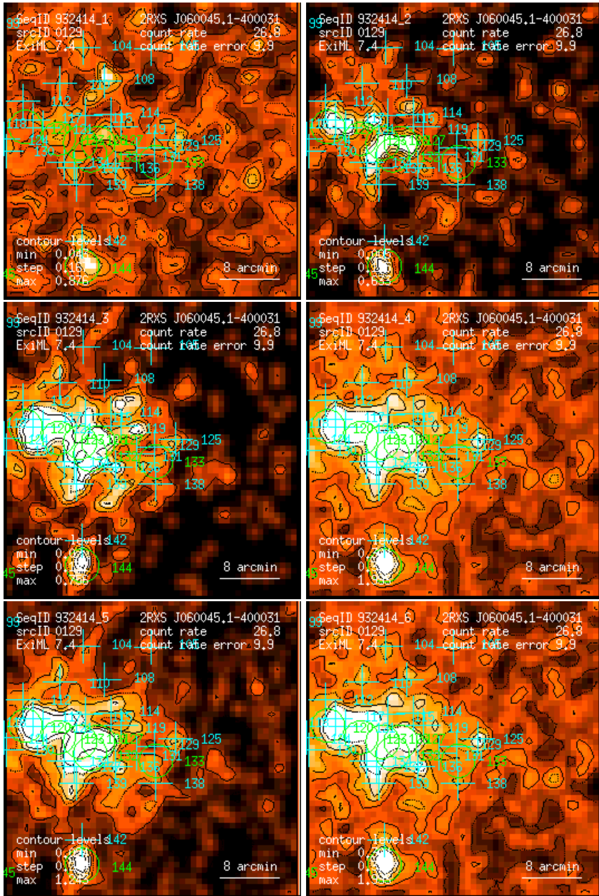
Figure 129: RASS 932414: detection 0129: band rate images, Gaussian filter: (1) PSPC channels 11 – 41, (2) 52 – 90, (3) 91 – 201, (4) 11 – 235, (5) 52 – 201, (6) 11 – 201. Broad band rates in counts/ks. Band rate contour levels in counts/ks/arcmin 2 .
