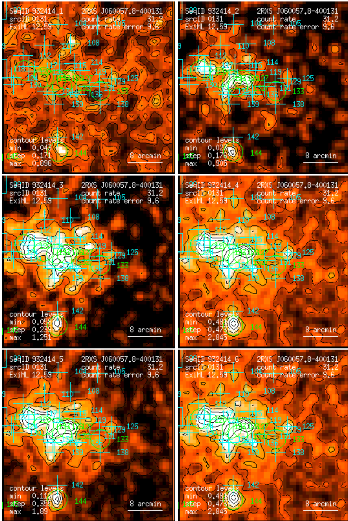
Figure 131: RASS 932414: detection 0131: band rate images, Gaussian filter: (1) PSPC channels 11 – 41, (2) 52 – 90, (3) 91 – 201, (4) 11 – 235, (5) 52 – 201, (6) 11 – 201. Broad band rates in counts/ks. Band rate contour levels in counts/ks/arcmin 2 .
