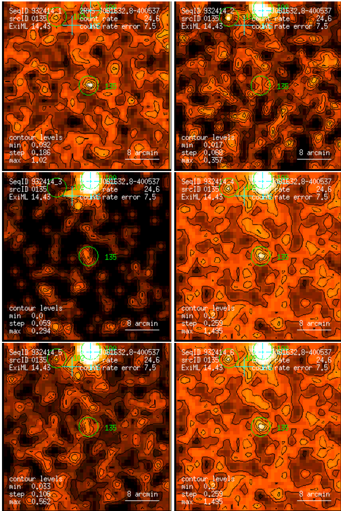
Figure 135: RASS 932414: detection 0135: band rate images, Gaussian filter: (1) PSPC channels 11 – 41, (2) 52 – 90, (3) 91 – 201, (4) 11 – 235, (5) 52 – 201, (6) 11 – 201. Broad band rates in counts/ks. Band rate contour levels in counts/ks/arcmin 2 .
