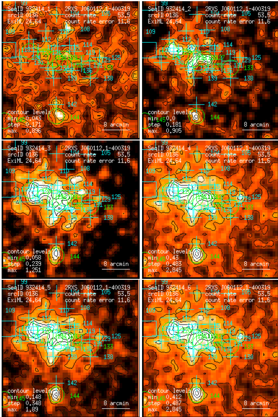
Figure 136: RASS 932414: detection 0136: band rate images, Gaussian filter: (1) PSPC channels 11 – 41, (2) 52 – 90, (3) 91 – 201, (4) 11 – 235, (5) 52 – 201, (6) 11 – 201. Broad band rates in counts/ks. Band rate contour levels in counts/ks/arcmin 2 .
