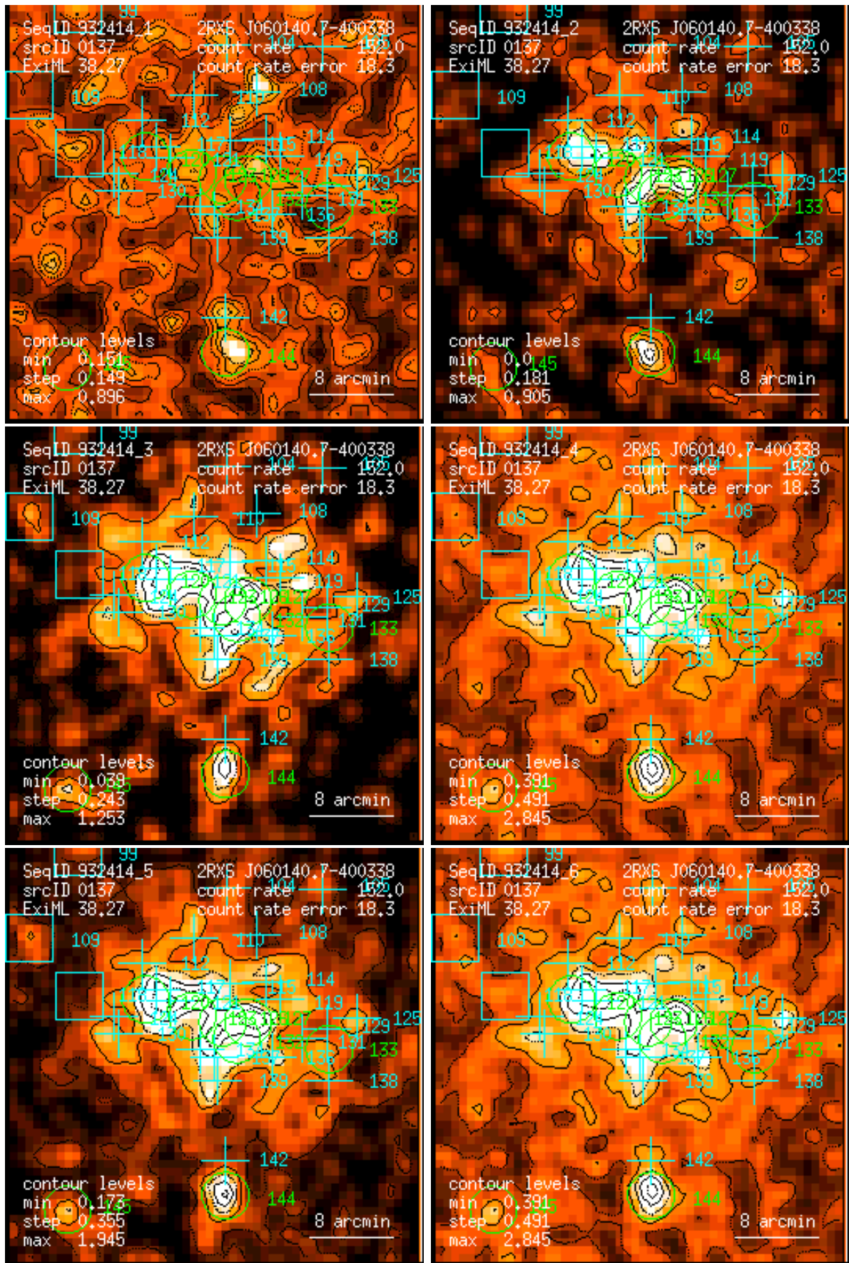
Figure 137: RASS 932414: detection 0137: band rate images, Gaussian filter: (1) PSPC channels 11 – 41, (2) 52 – 90, (3) 91 – 201, (4) 11 – 235, (5) 52 – 201, (6) 11 – 201. Broad band rates in counts/ks. Band rate contour levels in counts/ks/arcmin 2 .
