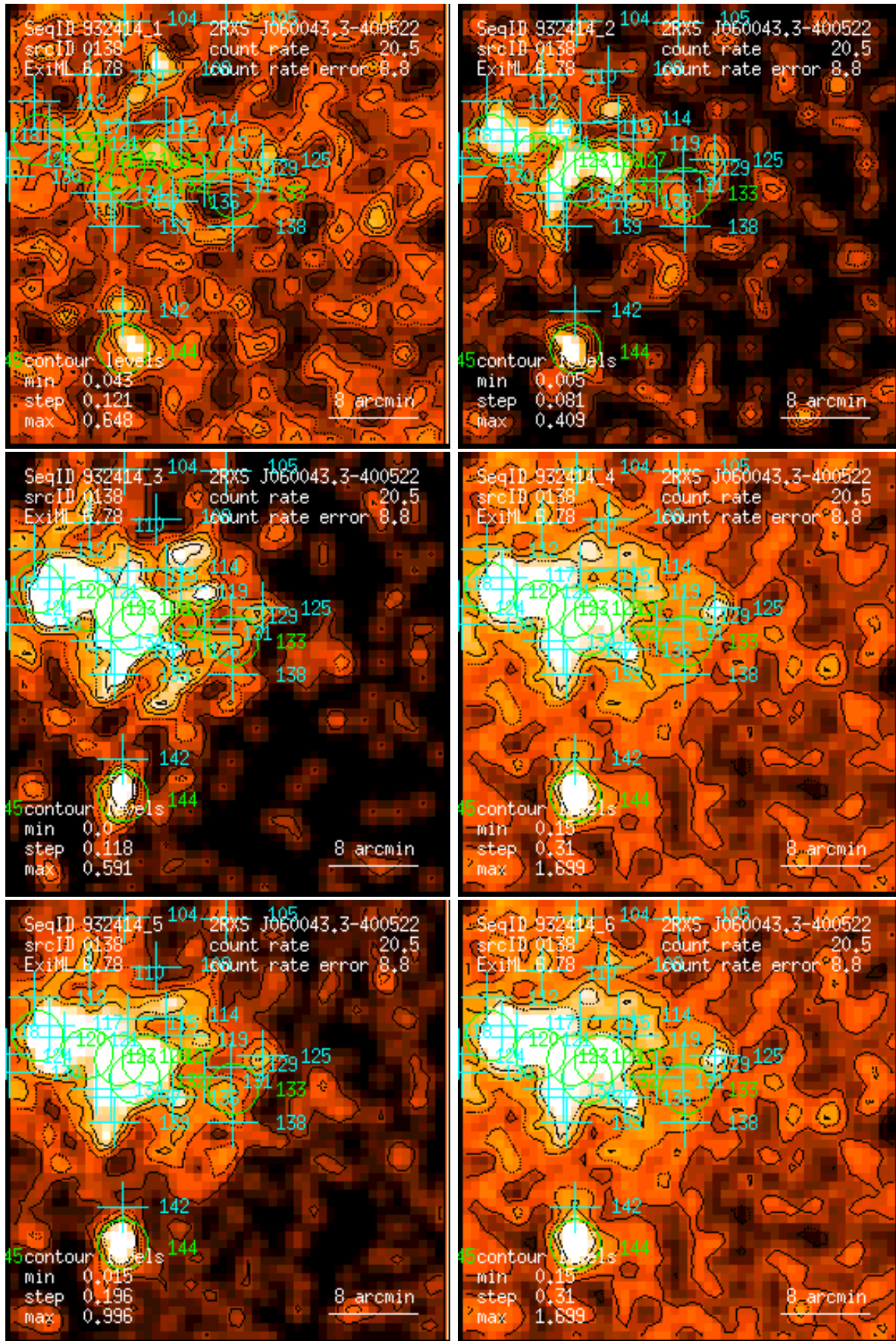
Figure 138: RASS 932414: detection 0138: band rate images, Gaussian filter: (1) PSPC channels 11 – 41, (2) 52 – 90, (3) 91 – 201, (4) 11 – 235, (5) 52 – 201, (6) 11 – 201. Broad band rates in counts/ks. Band rate contour levels in counts/ks/arcmin 2 .
