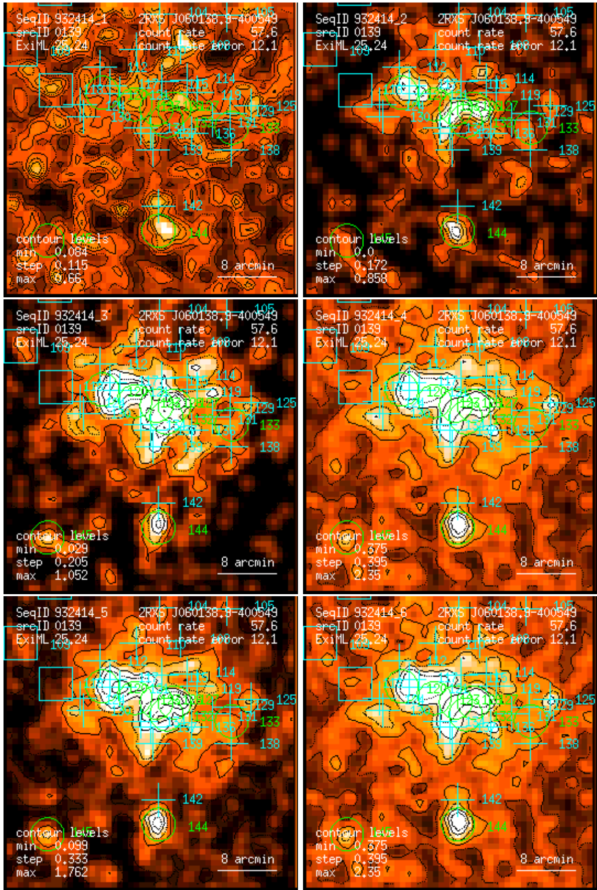
Figure 139: RASS 932414: detection 0139: band rate images, Gaussian filter: (1) PSPC channels 11 – 41, (2) 52 – 90, (3) 91 – 201, (4) 11 – 235, (5) 52 – 201, (6) 11 – 201. Broad band rates in counts/ks. Band rate contour levels in counts/ks/arcmin 2 .
