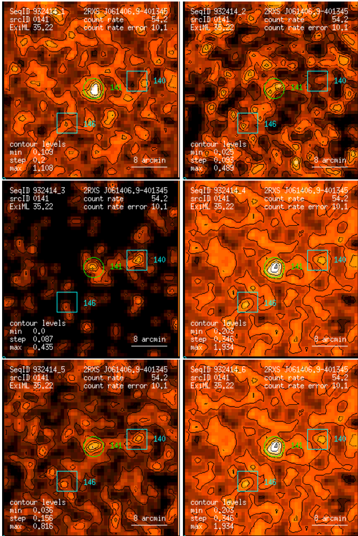
Figure 141: RASS 932414: detection 0141: band rate images, Gaussian filter: (1) PSPC channels 11 – 41, (2) 52 – 90, (3) 91 – 201, (4) 11 – 235, (5) 52 – 201, (6) 11 – 201. Broad band rates in counts/ks. Band rate contour levels in counts/ks/arcmin 2 .
