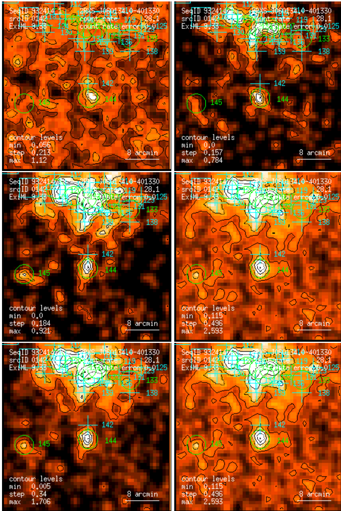
Figure 142: RASS 932414: detection 0142: band rate images, Gaussian filter: (1) PSPC channels 11 – 41, (2) 52 – 90, (3) 91 – 201, (4) 11 – 235, (5) 52 – 201, (6) 11 – 201. Broad band rates in counts/ks. Band rate contour levels in counts/ks/arcmin 2 .
