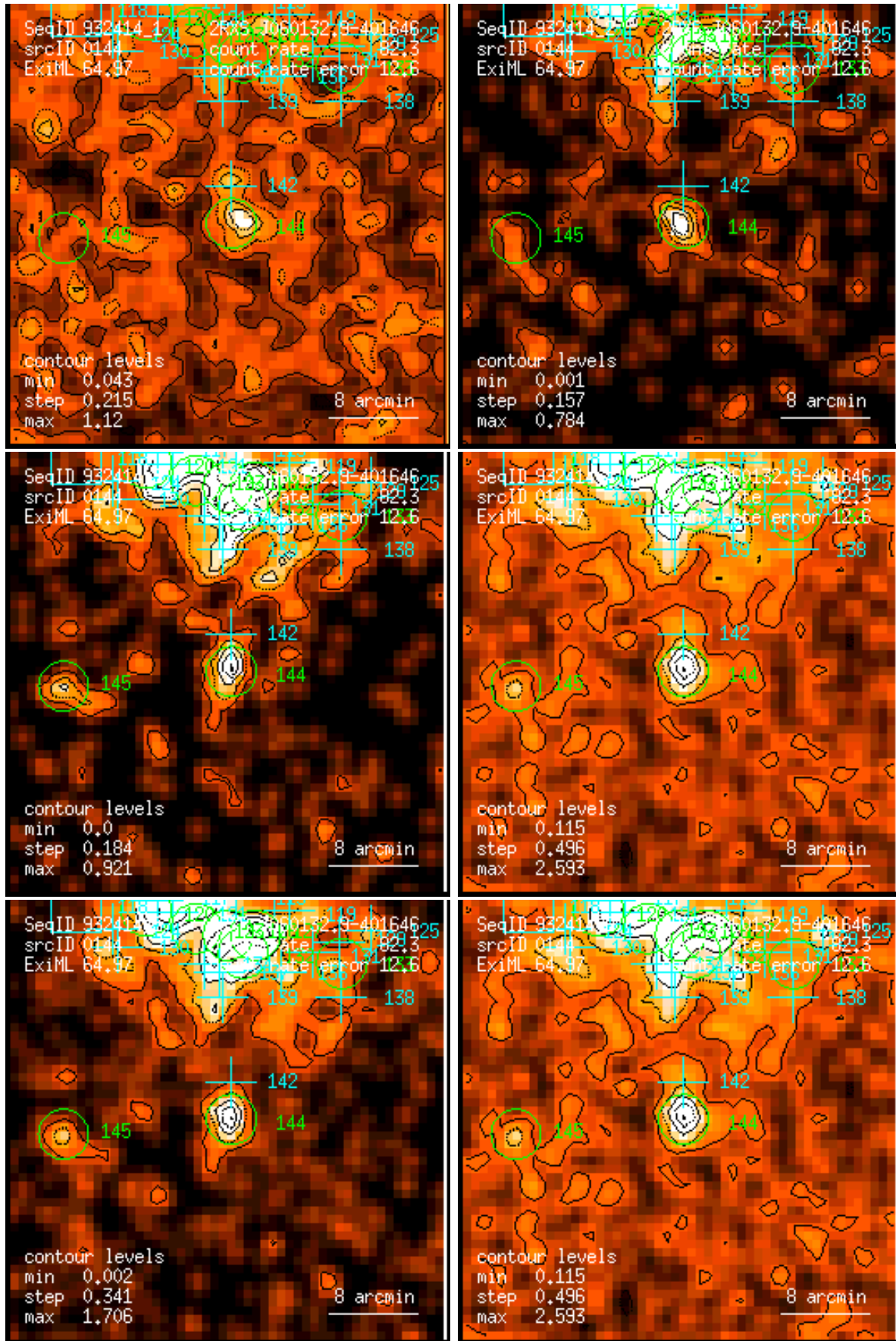
Figure 144: RASS 932414: detection 0144: band rate images, Gaussian filter: (1) PSPC channels 11 – 41, (2) 52 – 90, (3) 91 – 201, (4) 11 – 235, (5) 52 – 201, (6) 11 – 201. Broad band rates in counts/ks. Band rate contour levels in counts/ks/arcmin 2 .
