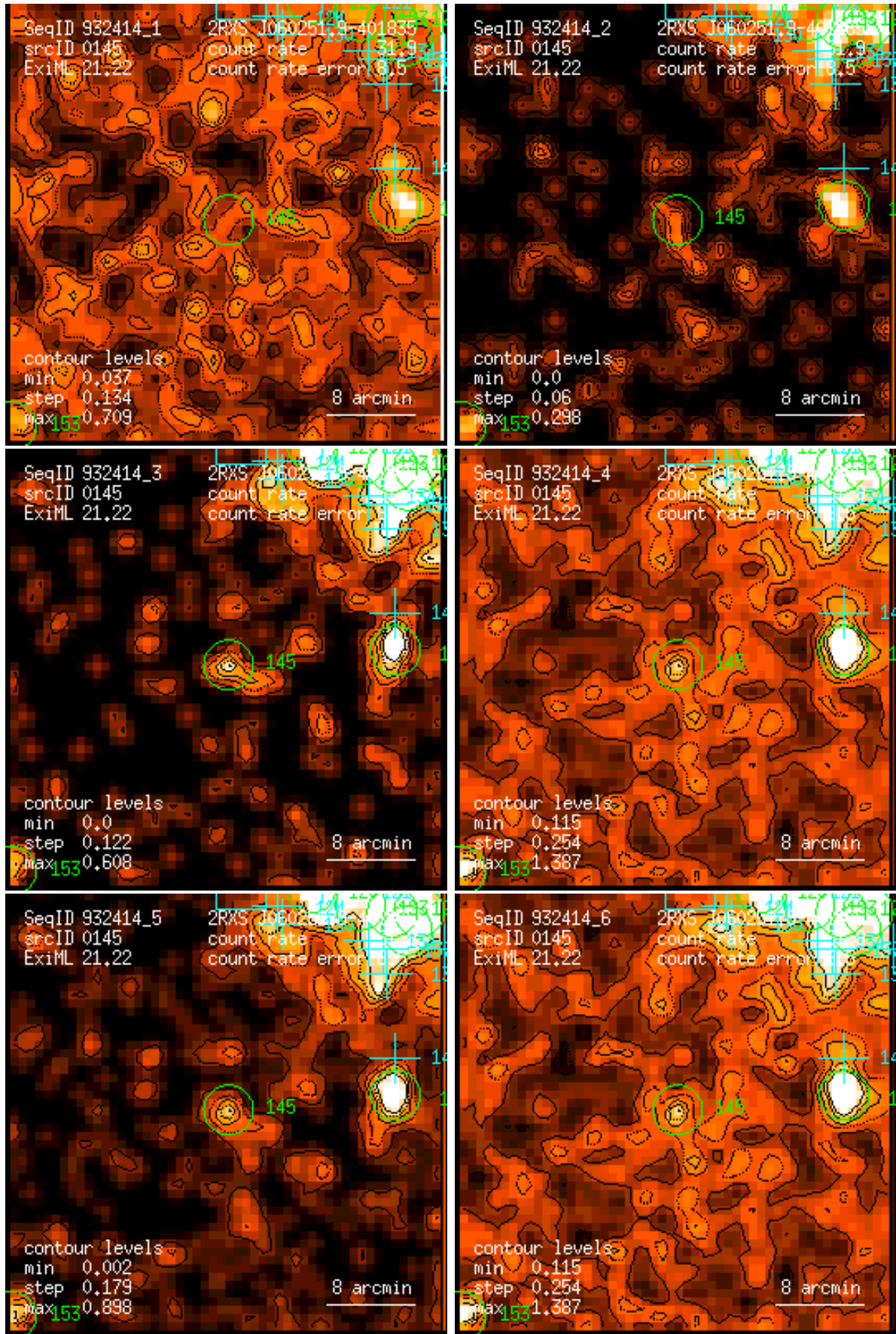
Figure 145: RASS 932414: detection 0145: band rate images, Gaussian filter: (1) PSPC channels 11 – 41, (2) 52 – 90, (3) 91 – 201, (4) 11 – 235, (5) 52 – 201, (6) 11 – 201. Broad band rates in counts/ks. Band rate contour levels in counts/ks/arcmin 2 .
