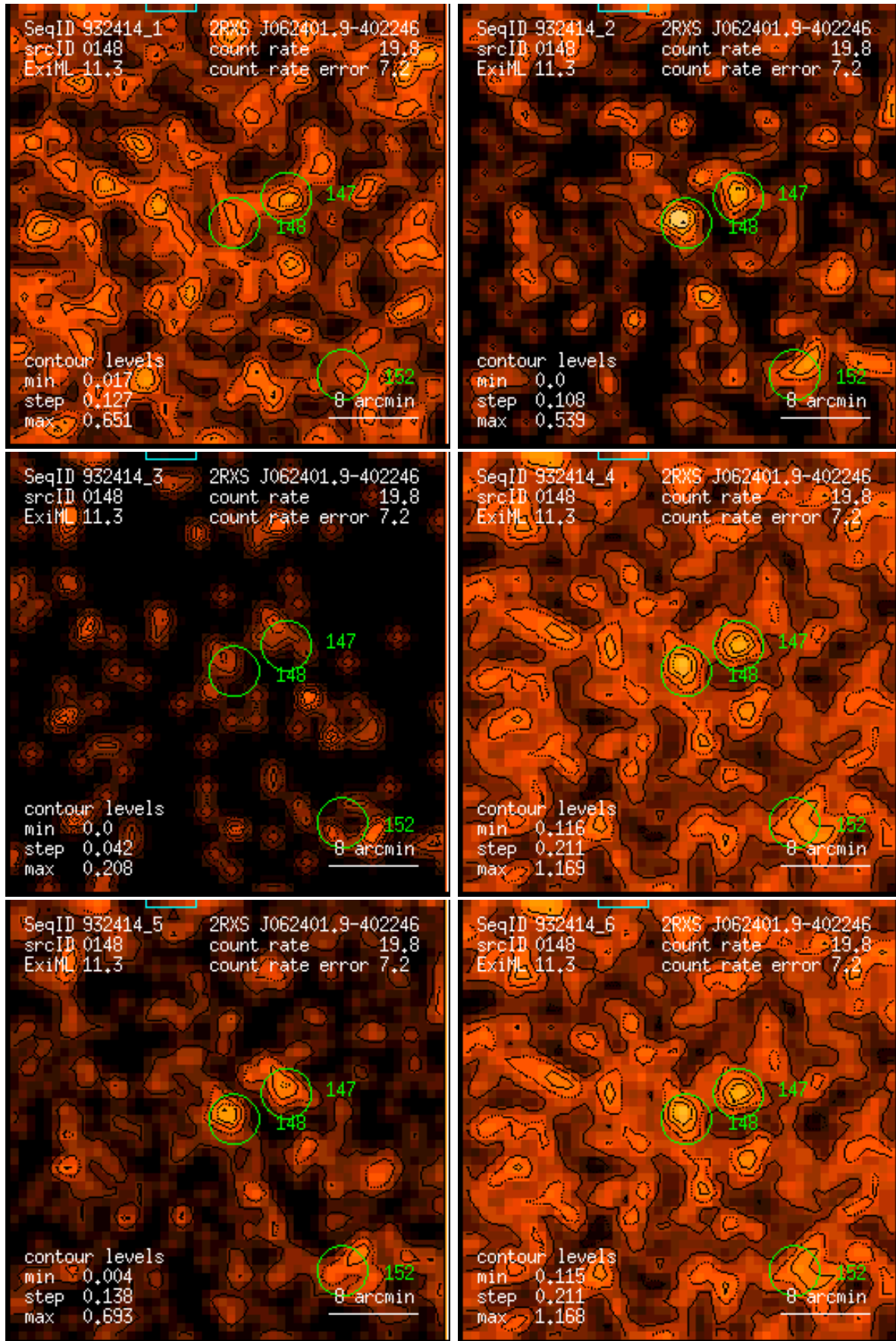
Figure 148: RASS 932414: detection 0148: band rate images, Gaussian filter: (1) PSPC channels 11 – 41, (2) 52 – 90, (3) 91 – 201, (4) 11 – 235, (5) 52 – 201, (6) 11 – 201. Broad band rates in counts/ks. Band rate contour levels in counts/ks/arcmin 2 .
