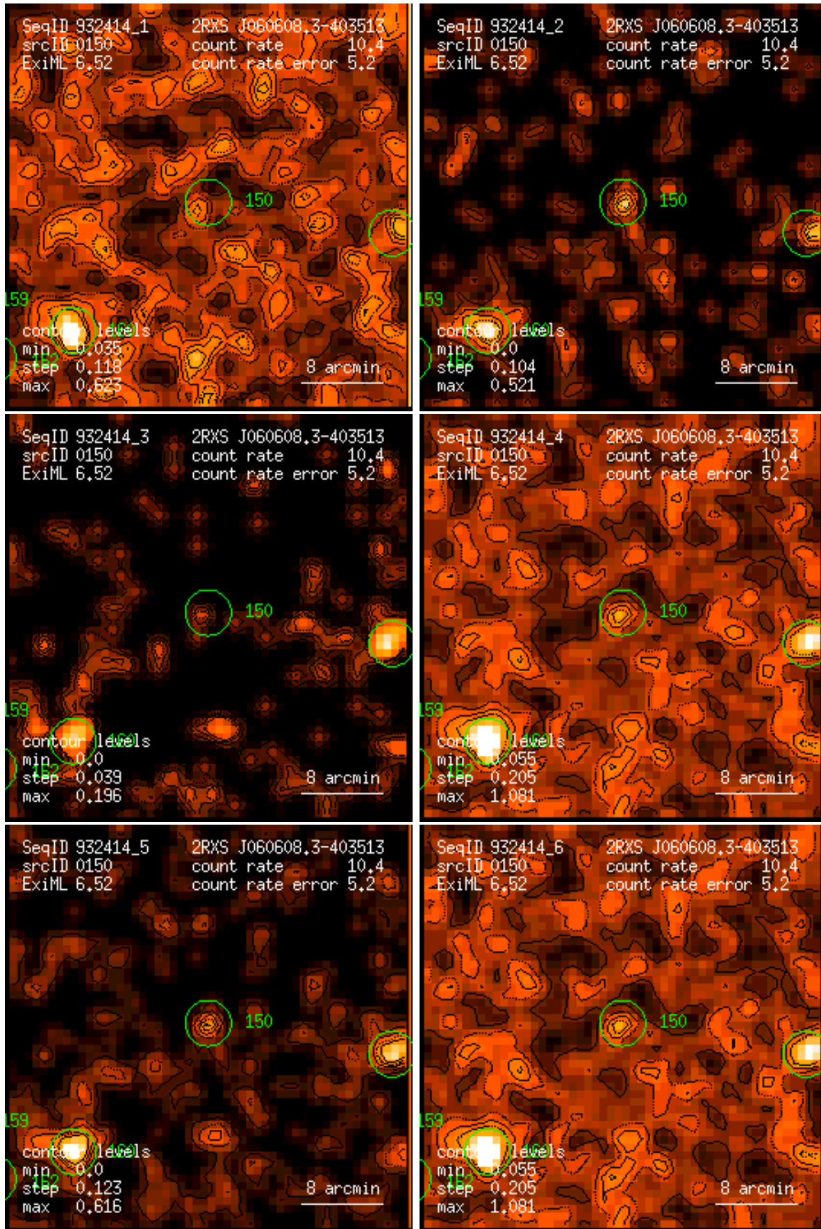
Figure 150: RASS 932414: detection 0150: band rate images, Gaussian filter: (1) PSPC channels 11 – 41, (2) 52 – 90, (3) 91 – 201, (4) 11 – 235, (5) 52 – 201, (6) 11 – 201. Broad band rates in counts/ks. Band rate contour levels in counts/ks/arcmin 2 .
