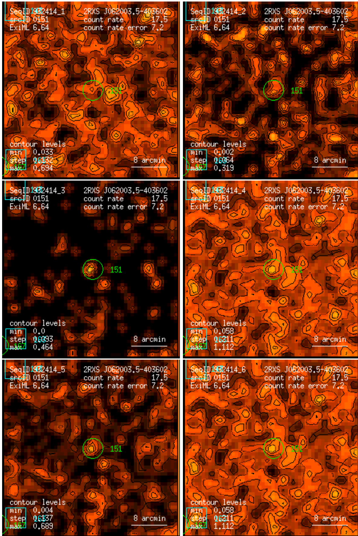
Figure 151: RASS 932414: detection 0151: band rate images, Gaussian filter: (1) PSPC channels 11 – 41, (2) 52 – 90, (3) 91 – 201, (4) 11 – 235, (5) 52 – 201, (6) 11 – 201. Broad band rates in counts/ks. Band rate contour levels in counts/ks/arcmin 2 .
