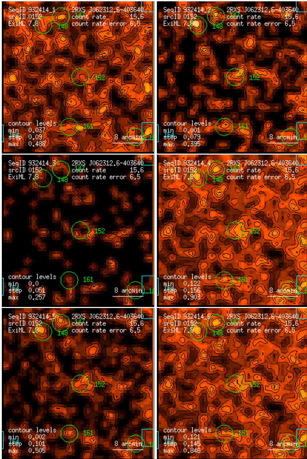
Figure 152: RASS 932414: detection 0152: band rate images, Gaussian filter: (1) PSPC channels 11 – 41, (2) 52 – 90, (3) 91 – 201, (4) 11 – 235, (5) 52 – 201, (6) 11 – 201. Broad band rates in counts/ks. Band rate contour levels in counts/ks/arcmin 2 .
