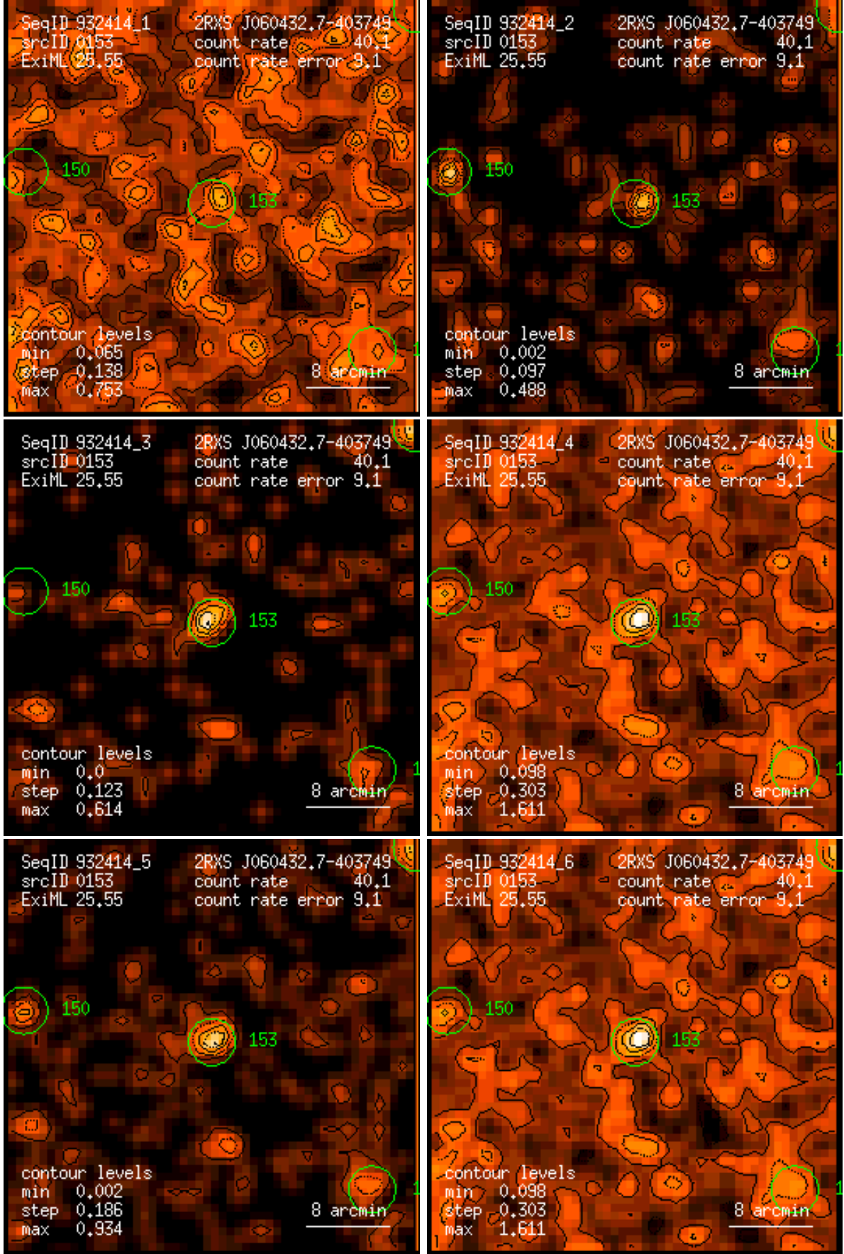
Figure 153: RASS 932414: detection 0153: band rate images, Gaussian filter: (1) PSPC channels 11 – 41, (2) 52 – 90, (3) 91 – 201, (4) 11 – 235, (5) 52 – 201, (6) 11 – 201. Broad band rates in counts/ks. Band rate contour levels in counts/ks/arcmin 2 .
