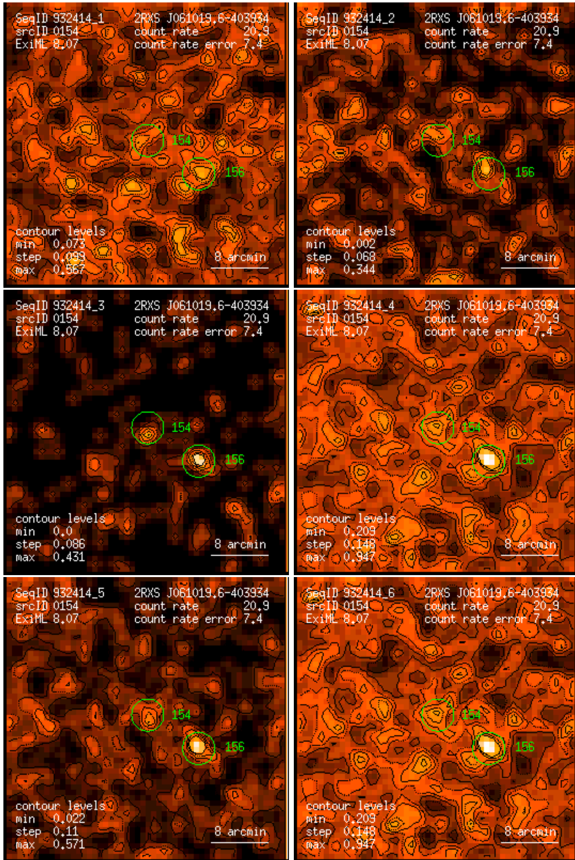
Figure 154: RASS 932414: detection 0154: band rate images, Gaussian filter: (1) PSPC channels 11 – 41, (2) 52 – 90, (3) 91 – 201, (4) 11 – 235, (5) 52 – 201, (6) 11 – 201. Broad band rates in counts/ks. Band rate contour levels in counts/ks/arcmin 2 .
