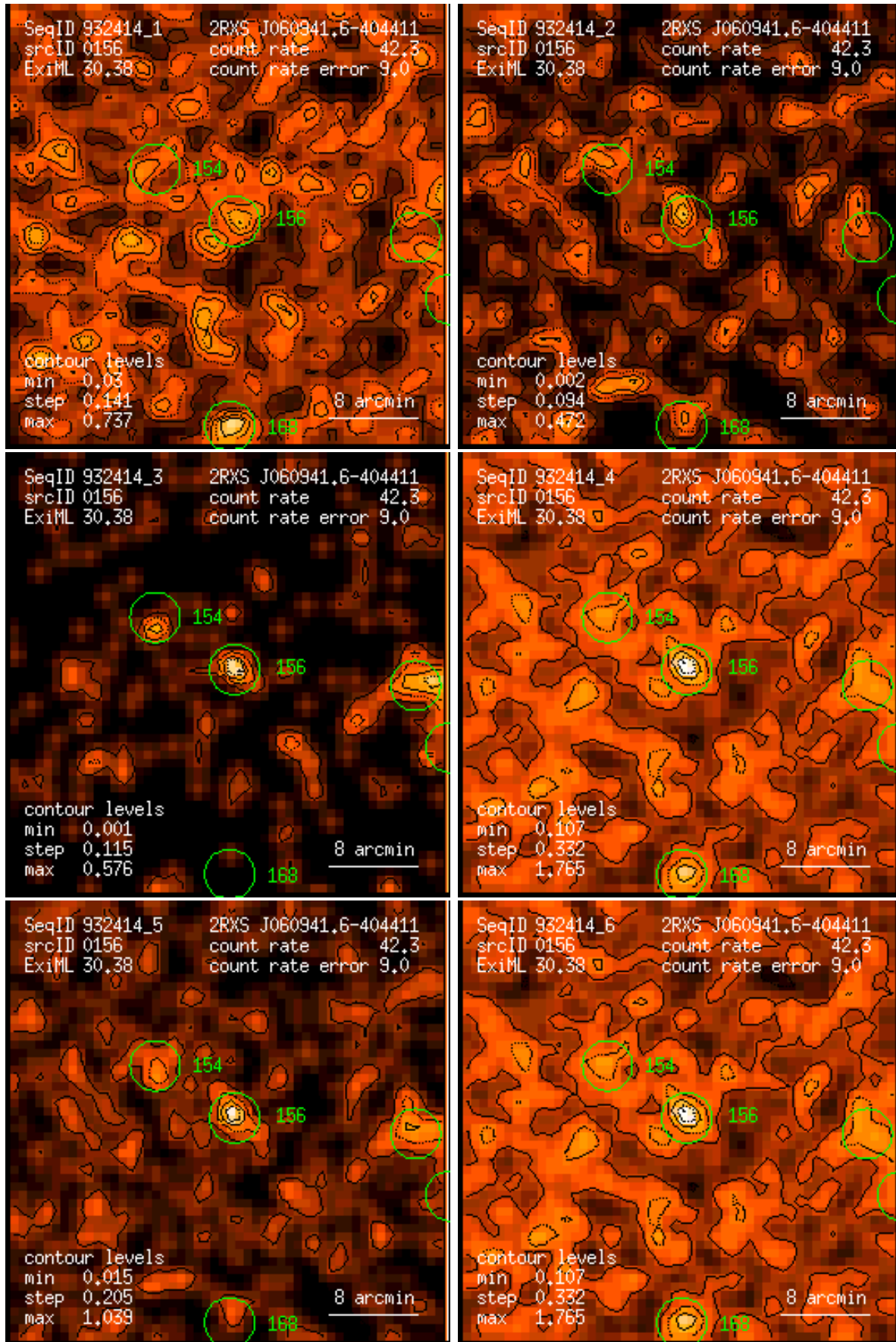
Figure 156: RASS 932414: detection 0156: band rate images, Gaussian filter: (1) PSPC channels 11 – 41, (2) 52 – 90, (3) 91 – 201, (4) 11 – 235, (5) 52 – 201, (6) 11 – 201. Broad band rates in counts/ks. Band rate contour levels in counts/ks/arcmin 2 .
