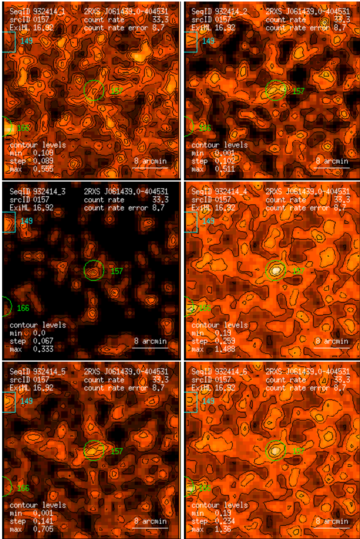
Figure 157: RASS 932414: detection 0157: band rate images, Gaussian filter: (1) PSPC channels 11 – 41, (2) 52 – 90, (3) 91 – 201, (4) 11 – 235, (5) 52 – 201, (6) 11 – 201. Broad band rates in counts/ks. Band rate contour levels in counts/ks/arcmin 2 .
