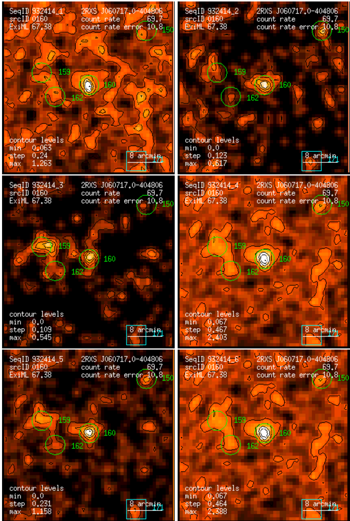
Figure 160: RASS 932414: detection 0160: band rate images, Gaussian filter: (1) PSPC channels 11 – 41, (2) 52 – 90, (3) 91 – 201, (4) 11 – 235, (5) 52 – 201, (6) 11 – 201. Broad band rates in counts/ks. Band rate contour levels in counts/ks/arcmin 2 .
