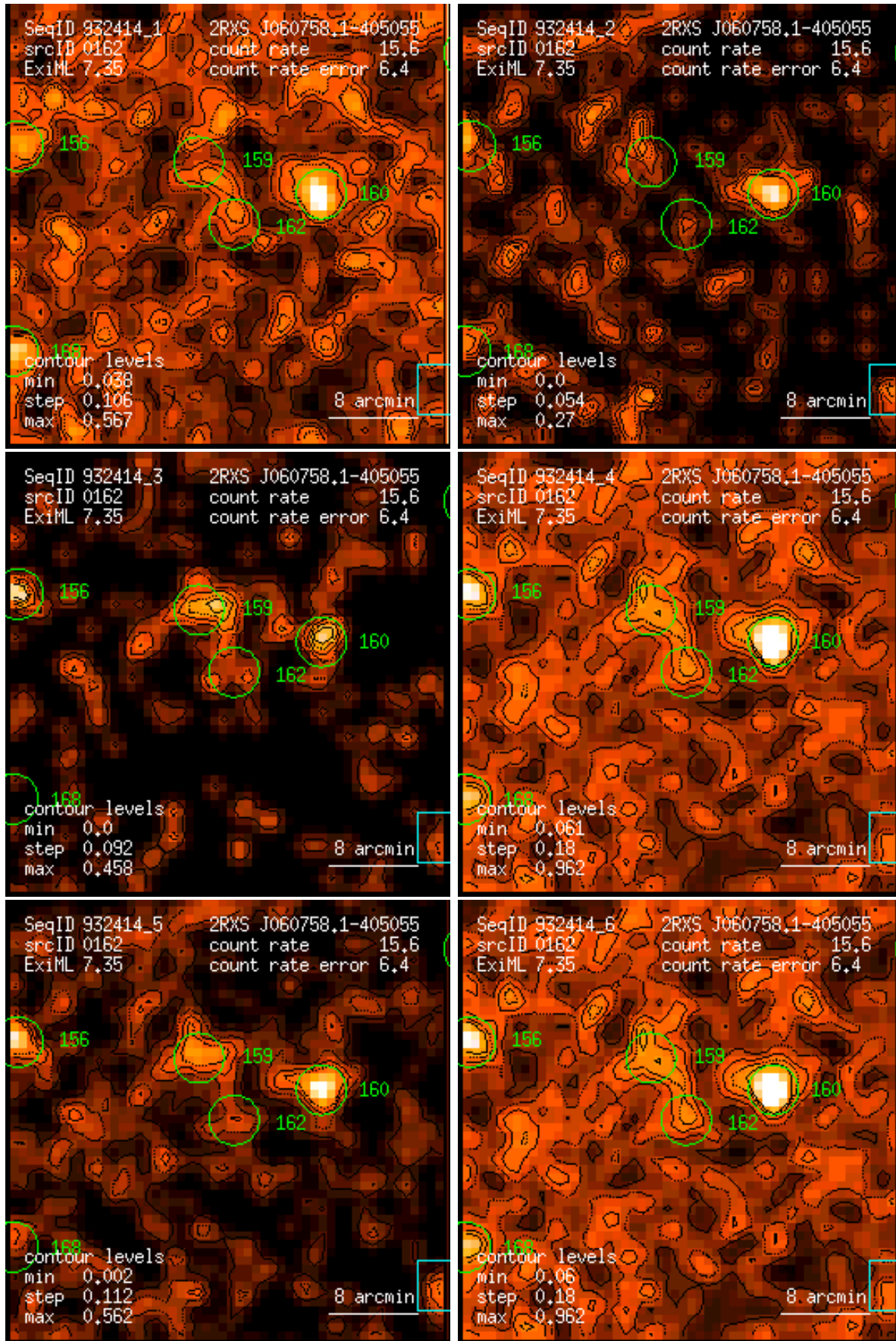
Figure 162: RASS 932414: detection 0162: band rate images, Gaussian filter: (1) PSPC channels 11 – 41, (2) 52 – 90, (3) 91 – 201, (4) 11 – 235, (5) 52 – 201, (6) 11 – 201. Broad band rates in counts/ks. Band rate contour levels in counts/ks/arcmin 2 .
