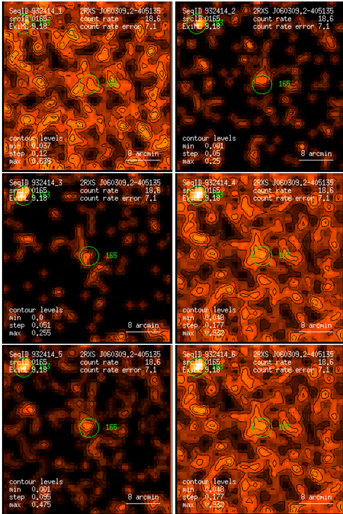
Figure 165: RASS 932414: detection 0165: band rate images, Gaussian filter: (1) PSPC channels 11 – 41, (2) 52 – 90, (3) 91 – 201, (4) 11 – 235, (5) 52 – 201, (6) 11 – 201. Broad band rates in counts/ks. Band rate contour levels in counts/ks/arcmin 2 .
